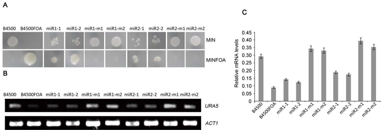
Figure 5. Silencing of the reporter gene URA5-miRs . (A) The upper panels show a slower growth rate of the transformants of URA5-miR1 (two transformants was picked in each case, namely, miR1-1 and miR1-2), and URA5-miR2 (miR2-1 and miR2-2), than the wild type B4500, and the transformants of miR1-m ( i.e. miR1-m1 and m2) and miR2-m, on MIN agar supplemented with 100 \mu g/ml hygromycin B, no hygromycin for B4500 and B4500FOA. The negative control B4500FOA ( ura5 ) did not grow on MIN. On MINFOA (the bottom panels), the wild type strains and transformants of miR1-m and miR2-m were killed by FOA. Transformants containing miR1 and miR2, as well as ura5 - strain B4500FOA grew properly. MIN: minimal medium, and MINFOA: minimal medium with 5-FOA and 50 mg/l uracil. For selection of transformants, 100 \mu g/ml hygromycin B was added to MIN or MINFOA when needed. (B) Reverse transcription-PCR confirmed the decreased mRNA level of URA5 in URA5-miR transformants. URA5 mRNA levels in the wild type and in the transformants of miR-ms were close to each other. In each assay, two transformants were picked for double examination. (C) A semi-quantification of URA5 mRNA to ACT1 mRNA in the strains in (B). doi:10.1371/journal.pone.0052734.g005
