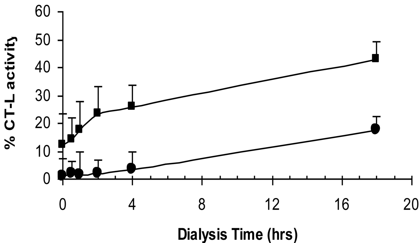
Figure 3. Recovery of CT-L activity upon dialysis of the 20S proteasome-compound complexes after pre-incubation with PI-083 (■) and Bortezomib (●).
