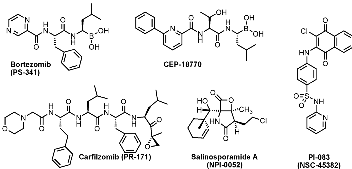
Figure 1. Proteasome inhibitors; Bortezomib (clinically approved covalent and reversible inhibitor). CEP- 18770 (reversible inhibitor), carfilzomib and salinosporamide A (irreversible inhibitors) currently in phase I and II clinical trials. PI-083 (reversible inhibitor identified from the NCI diversity set-1).
