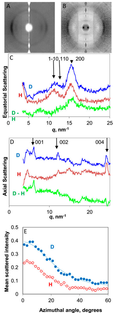
Figure 3. WANS from celery collenchyma cell walls. A, Scattering patterns in H form (right half) and after deuteration exchange of hydroxyl groups accessible to water (left half). The fiber axis is vertical. B, Difference scattering pattern (D – H). C, Equatorial scattering profiles from cell walls in H form, D form, and difference (D – H). D, Scattering profiles on the fiber axis from cell walls in H form, D form, and difference (D – H). E, Azimuthal scattering profiles across the 200 reflection. [See online article for color version of this figure.]
