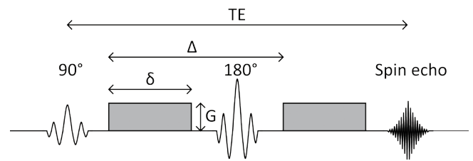
Figure 2 Pulsed gradient spin echo NMR sequence. The spin echo sequence is modified by the addition of two gradient pulses (grey blocks) which induce and then reverse a spatially-dependent phase shift
