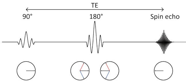
Figure 1 Spin echo NMR sequence. The 90 degree RF pulse produces coherent transverse magnetization (first circle). The spins begin to dephase due to magnetic field inhomogeneities (red, blue and black arrows in the second circle). The 180 degree pulse reverses the phase dispersal (third circle). The spins then rephase and produce an echo (fourth circle)
