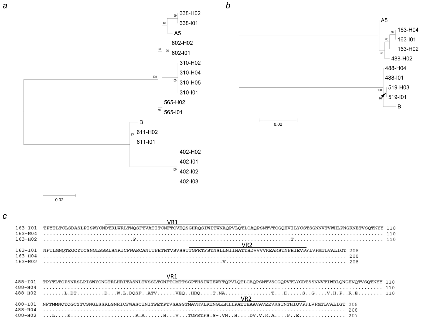
Figure 3. Alignment of K1 sequences from members of nine households where sequence data was obtained from the index child and at least one other household member. Maximum likelihood phylogenetic tree of K1 nucleotide sequence from individuals indicating intra-household (a) and extra-household (b) transmission of KSHV to children. (c) K1 amino acid alignment for individuals of households 163 and 488. H02 designates the mother in each household.
