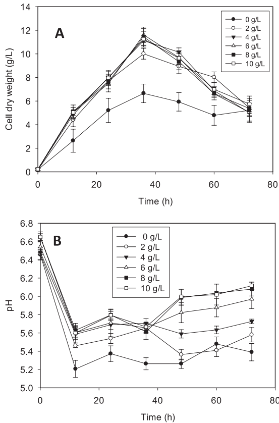
FIG 1 Comparative cell dry weight (A) and pH (B) profiles of C. beijerinckii ABE fermentation in P2 medium supplemented with the indicated concentrations of CaCO 3 .
