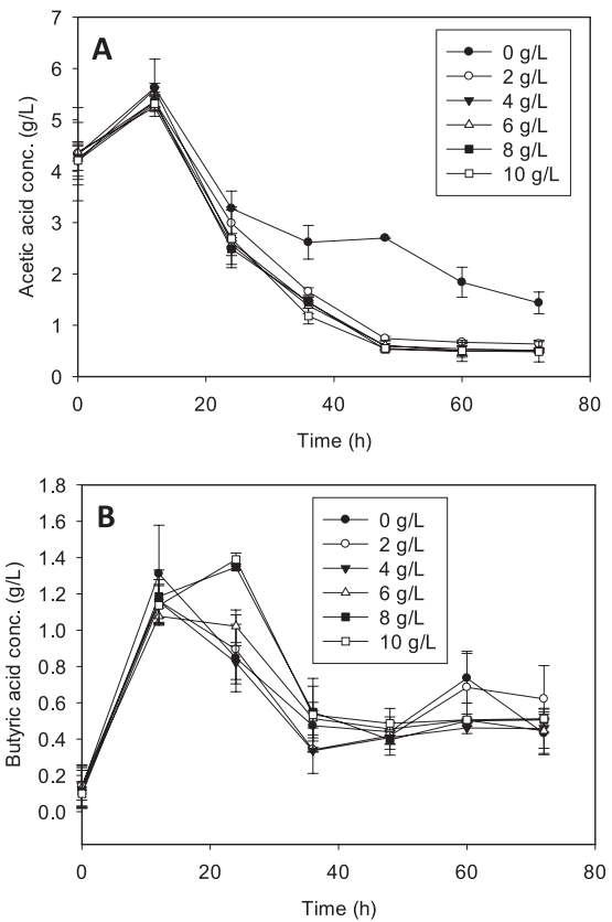
FIG 2 Acetic (A) and butyric (B) acid concentrations in the fermentation medium of C. beijerinckii grown in P2 medium and P2 medium supplemented with the indicated concentrations of CaCO 3 .
