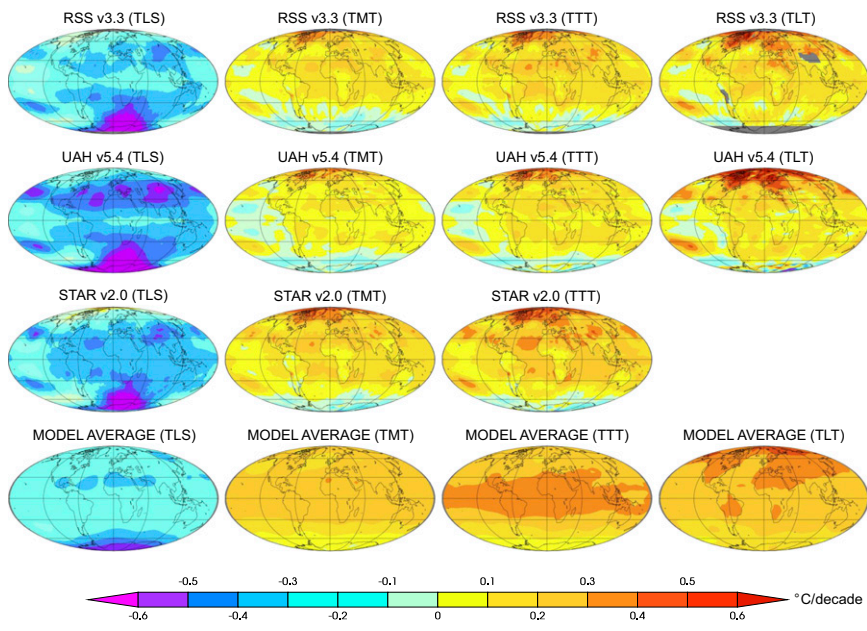
Fig. 4. Geographical patterns of observed and simulated trends (in degrees Celsius per decade) in TLS, TMT, TTT, and TLT (columns 1–4, respectively). All trends are from 1979 to 2011. Simulated trends are the O3+V multimodel averages of synthetic MSU temperature changes from the spliced historical/RCP8.5 runs. Gray shading denotes areas where temperature information is not provided ( SI Appendix ).
