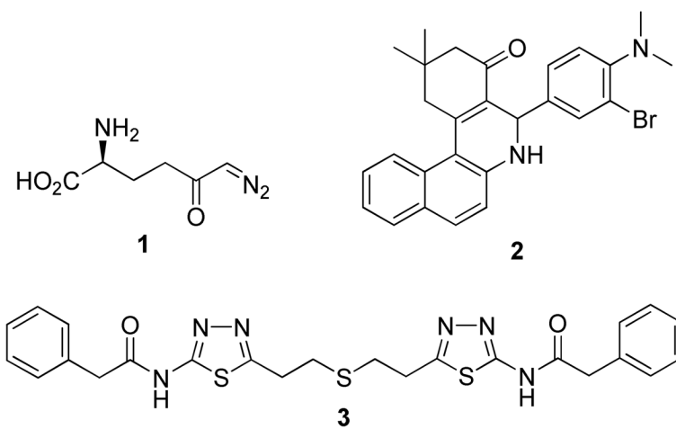
Figure 1. Structures of representative GLS inhibitors
