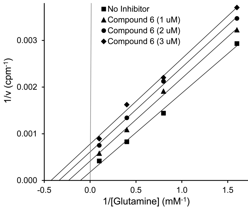
Figure 3. Double-reciprocal plot of the hydrolysis of glutamine by GLS1 in the presence of compound 6 . The straight lines represent the least squares fit of the data obtained by plotting the reciprocal of glutaminase activity versus the reciprocal of the glutamine concentrations.
