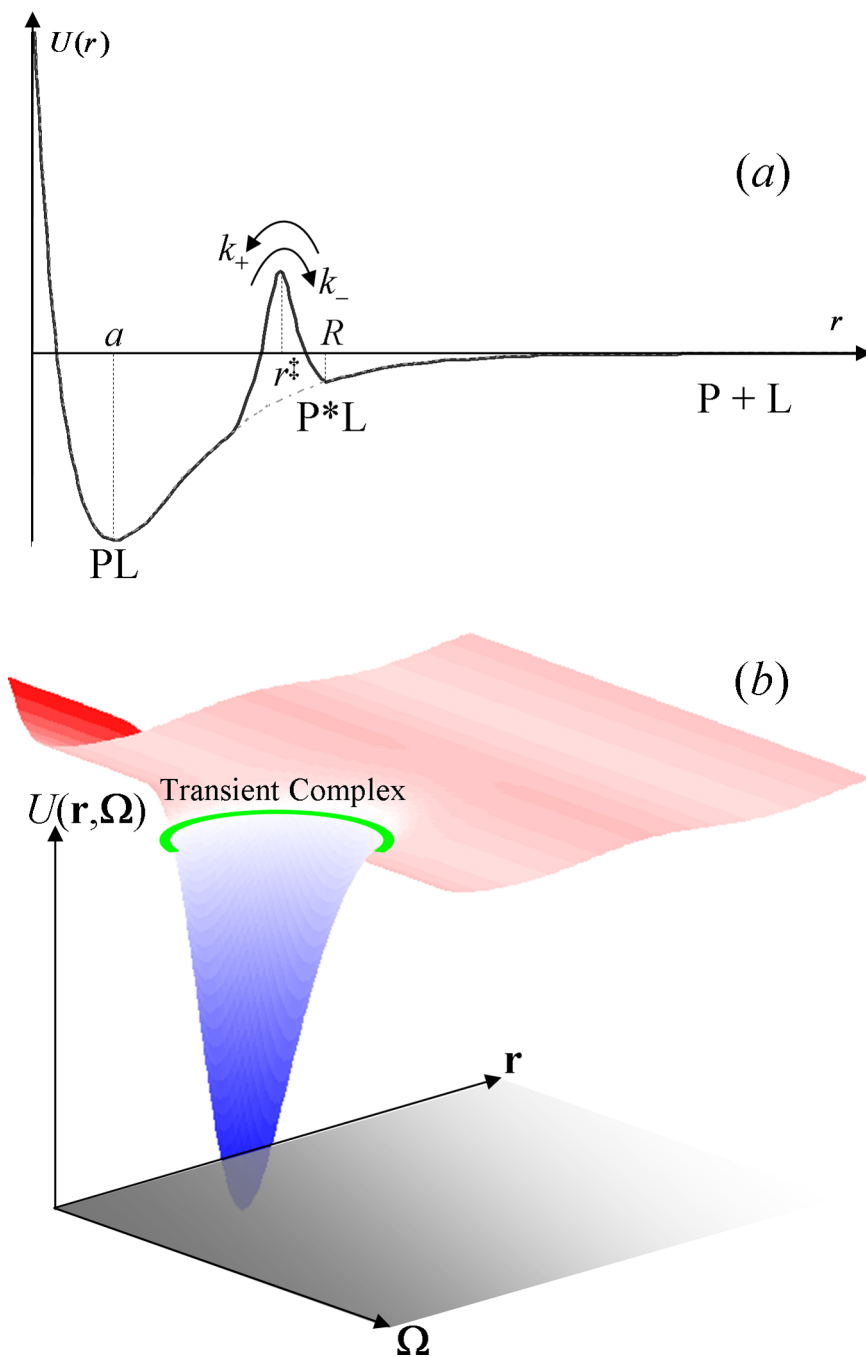
Fig. 4. Interaction energy functions. (a) Centrosymmetric model. The solid curve shows the energy function, with locations of the unbound state (i.e., P + L), transient complex (i.e., P*L), transition state, and native complex (i.e., PL) identified. The dashed curve is after smoothing out the transition state. (b) A smoothed energy function in relative translational ( \mathbf{r} ) and rotational ( \Omega ) space. The native complex is located in the deep well; the transient complex is located at the outer boundary of the energy well.
