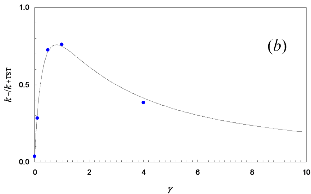
Fig. 3. A one-dimensional model for unimolecular reaction. (a) The potential energy function. (b) Results for the rate constant obtained from computer simulations (filled circles) and predicted by Melnikov and Meshkov [Eqs. (3.69) and (3.71); curve], for the potential energy function U(x) = (x^2 - 1)^2 , with k_B T = 1/4 and m = 1 . The simulations results are from Zhou (1989), by fitting the number correlation function [Eq. (3.20)] to an exponential function.
