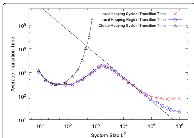
Figure 9 Average transition time from dead state to living state as function of system size with parameters set as: m=5, s=10, a=10, r_0=0.02, k=2, u=1, h=50, f=1 . The straight line illustrates a scaling of 1/L^2 .
