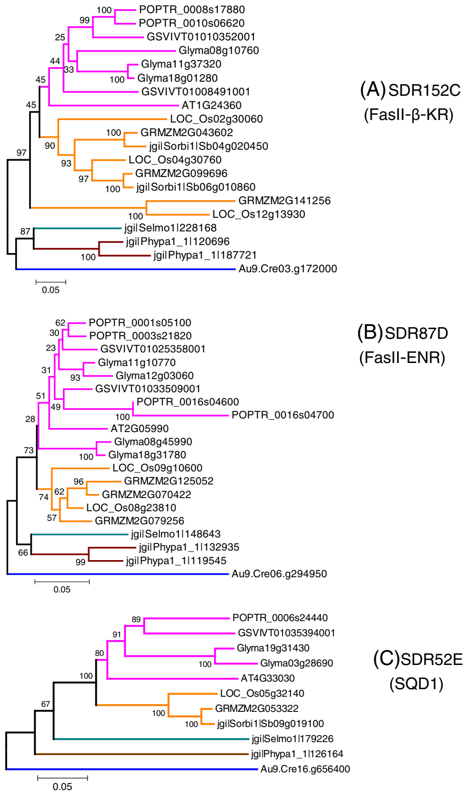
Figure 7 Phylogenetic trees of three families involved in lipid primary metabolism. (A) SDR152C-FasII-β-keto-reductase (β-KR); (B) SDR87D-FasII-Enoyl-ACP-reductase (ENR); (C) SDR52E UDP-sulfoquinovose synthase (SQD1). Amino acids sequences recognized by the SDR152C, SDR87D and SDR52E HMMs were aligned with ClustalW algorithm. The evolutionary history and the bootstrap test (500 replicates) were computed as described for SDR108E (Figure 3).
