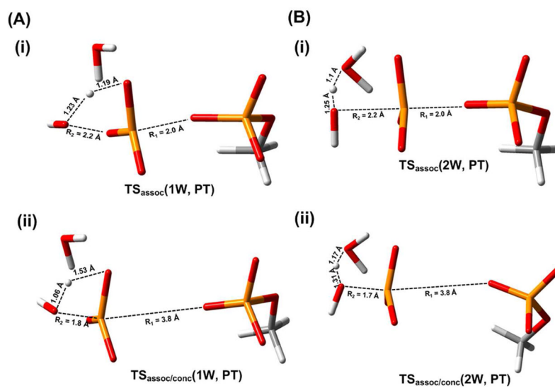
Figure 9. The geometric features of the key transition states corresponding to the 1W and 2W pathways following the associative and associative/concerted mechanisms.
