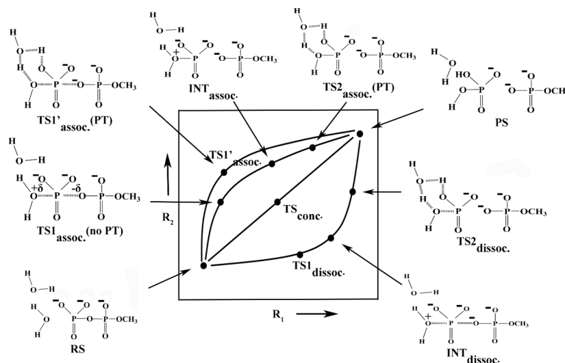
Figure 3. A schematic description of the potential energy surface for the hydrolysis of monomethyl pyrophosphate trianion utilizing the water assisted PT mechanism. The pathways corresponding to the associative, dissociative, and concerted mechanisms are clearly defined and the representative geometries corresponding to the key characteristic points along the potential energy surface are also depicted.
