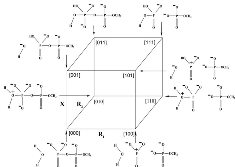
Figure 6. Schematic three-dimensional representation of the hydrolysis of monomethyl pyrophosphate trianion along the three reaction coordinates R_1 , R_2 , and X . [000] , and [111] represents the RS, and PS states respectively. [100] , [010] , and [001] are the states representing where the reaction had proceeded only along that respective reaction coordinate. [110] , [101] , and [011] corresponds to the states where the reaction had occurred along the respective two reaction coordinates.
