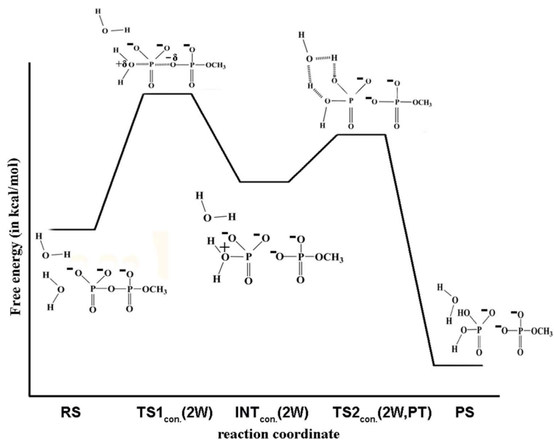
Figure 4. Schematic diagram of the free energy surface and the representative geometries for the hydrolysis of monomethyl pyrophosphate trianion in solution following the catalytic mechanism explored in Ref. 11 This mechanism corresponds to the associative (2W) pathway depicted in Fig. 5.
