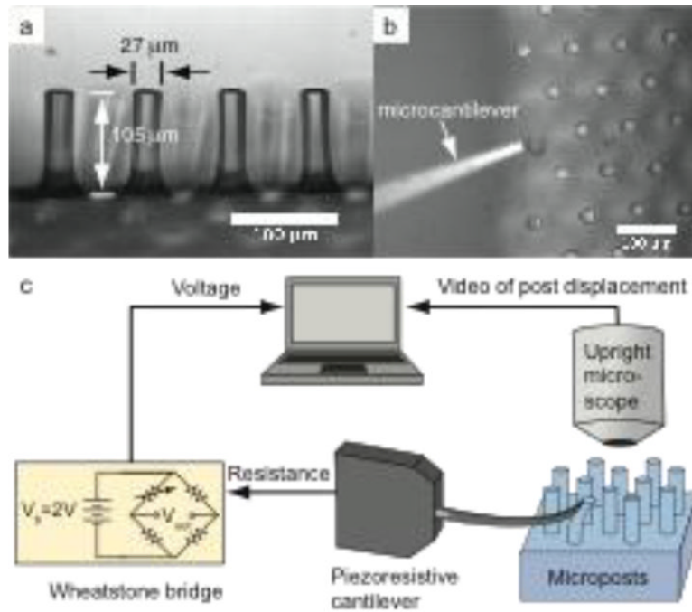
Fig. 3. Microposts (a) are calibrated using a piezoresistive microcantilever (b). Force is calculated from voltage out of the Wheatstone bridge and displacement is measured optically using an upright microscope (c). Scale bar represents 100 μm. Panels A and B adapted from (Taylor et al. 2010)
