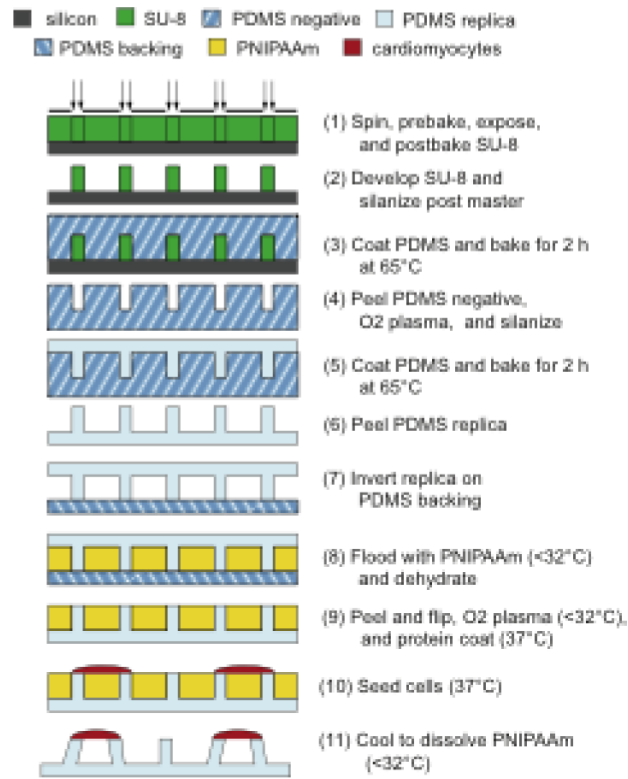
Fig. 2. Device fabrication starts with replica molding of microposts (steps 1–6) followed by inversion of the replica on a PDMS backing (step 7), deposition of the thermoresponsive sacrificial layer (steps 8–9), cell seeding (step 10), and dissolution of the sacrificial support layer (step 11)
