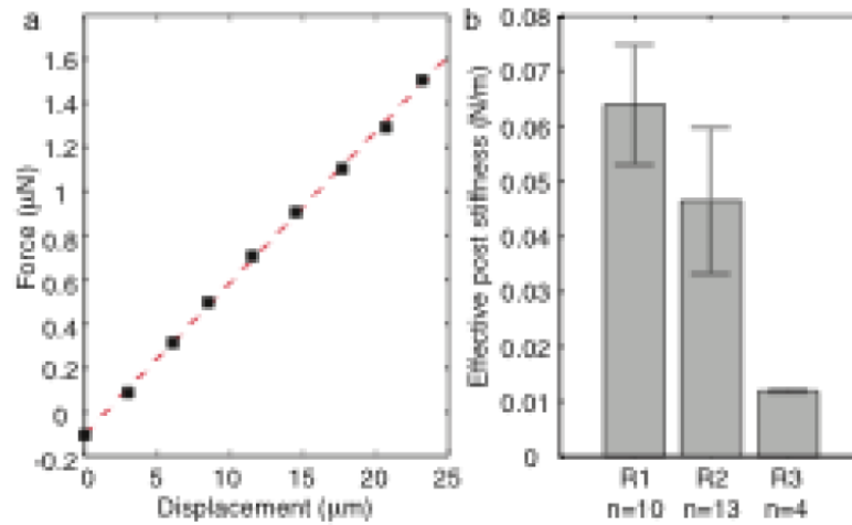
Fig. 5. Force-displacement curves (a) for each micropost verify linearity within the desired measurement range up to 20 \mu\text{m} . Each device was made from a separate batch of PDMS according to the same recipe, and multiple posts were calibrated to determine device stiffness, which varied considerably from batch to batch (b). Error bars represent standard deviation
