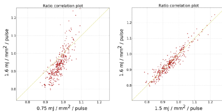
Fig. 1. Correlation plots between the ratios of 10^\circ data sets at different laser exposure collected at 90K. The yellow line has a 45^\circ slope. Only data observed on all 10 repeated frames were included.
