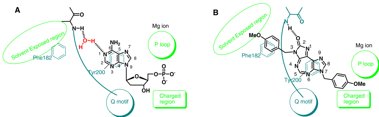
Figure 2. (A) Model for interactions between AMP and DDX3 (B) Proposed model for interactions between 1 and DDX3.
