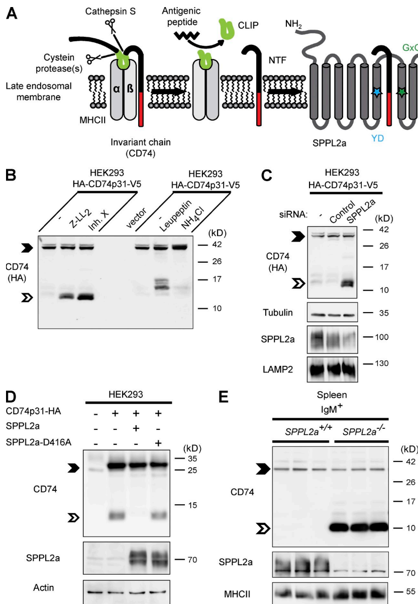
Figure 1. The intramembrane protease SPPL2a cleaves CD74 NTF. (A) Scheme of proteolytic degradation of CD74 in MHCII compartments, where the luminal domain is removed in a stepwise fashion by endosomal proteases and finally released from the MHCII dimer by cathepsin S. A small fragment (CLIP) persists inside the peptide-binding groove of MHCII, which is subsequently replaced with an antigenic peptide before the MHCII-peptide complex is transported to the plasma membrane. The remaining transmembrane NTF (82 aa) of CD74 is then proteolyzed by SPPL2a. The catalytically critical YD and GxGD motifs of SPPL2a are indicated by colored asterisks. (B) HEK293 cells stably expressing the p31 isoform of CD74 (HA-CD74p31-V5) were treated with 10 \mu M (Z-LL) 2 -ketone, 1 \mu M inhibitor X, 100 \mu M leupeptin or 25 mM NH 4 Cl for 5 h. The CD74 NTF is indicated by the open arrowheads. Full-length CD74 (closed arrowheads) and CD74 NTF were detected with anti-HA recognizing the epitope tag fused to the N terminus of the protein. (C) Transient knockdown of SPPL2a in HEK293 cells stably expressing HA-tagged CD74 (HA-CD74p31-V5). SPPL2a and the lysosomal membrane protein LAMP2 as control were analyzed in carbonate-washed membranes from the same batch of cells for enhancing SPPL2a detectability. (D) SPPL2a or the inactive D416A mutant were transiently co-expressed with CD74, followed by detection with anti-CD74 (In-1). (E) Using an antibody against an N-terminal epitope of CD74, endogenous CD74 was analyzed in splenic IgM + B cells isolated from SPPL2a -/- and control mice. (B-E) Electrophoretic separation before detection of CD74 was performed by standard Tris-Glycine SDS-PAGE (D) or using a Tris-Tricine buffer system (B, C, and E) with improved resolution in the low-molecular weight range. Equal protein loading was confirmed as indicated. Data are representative of three independent experiments.
