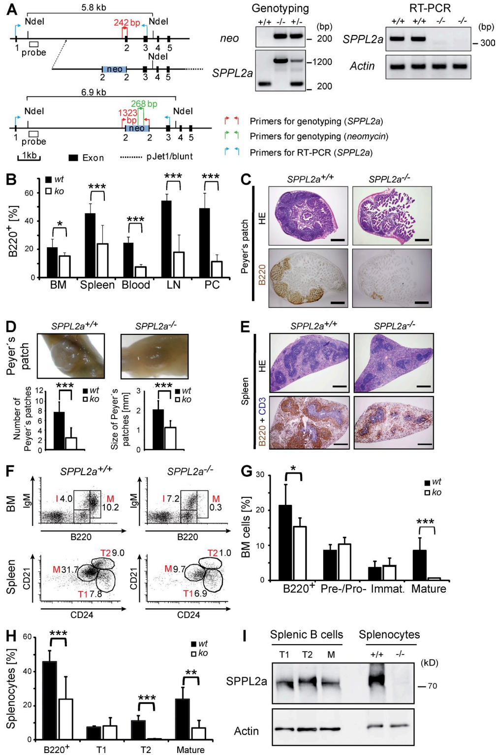
Figure 2. SPPL2a deficiency leads to impaired B cell development and function. (A) Generation of SPPL2a-deficient mice. The exon–intron structure of the murine SPPL2a gene, layout of the targeting construct, and structure of the targeted locus are depicted. Positions of primers and probes used for genotyping by PCR and Southern blot, respectively, are indicated. Genotyping of SPPL2a -/- mice was performed by PCR. DNA isolated from SPPL2a +/+ and SPPL2a -/- tail biopsies was amplified with either gene-specific ( SPPL2a ) or neomycin -specific primers. Total RNA was isolated from SPPL2a +/+ and SPPL2a -/- murine embryonic fibroblasts. After reverse transcription, primers annealing in exon 1 and exon 3 of the SPPL2a ORF as indicated were used to amplify a 342-bp fragment of the SPPL2a wild-type ORF from the cDNA. In parallel, appropriate primers for a fragment of \beta -actin were used as control.
