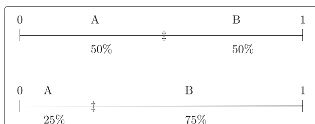
Figure 1 Probability boundaries for a two group randomization. First group is a 1:1 allocation to either group at a point where there are equal numbers in each group. The second is an example of a 1:3 allocation in favour of group B.
