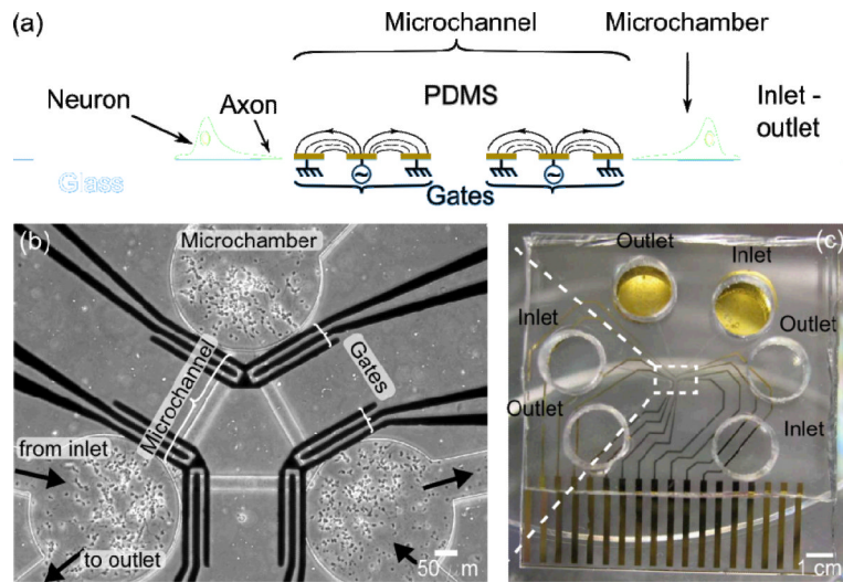
Fig. 4. (a) Side-view schematic of axon diode. (b–c) Images of axon diode chip showing three microchambers and electrodes.
