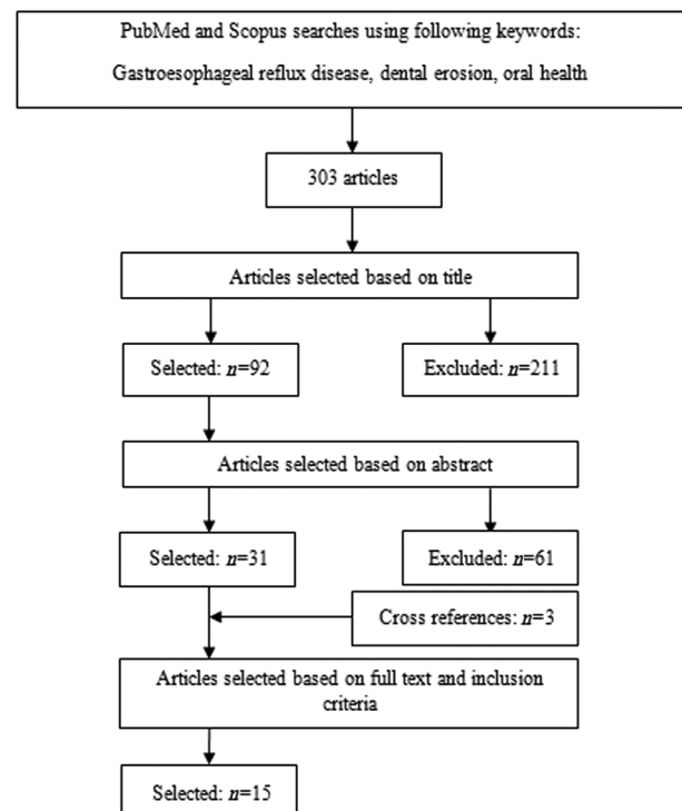
Figure 1: Diagram of the systematic review and searches
