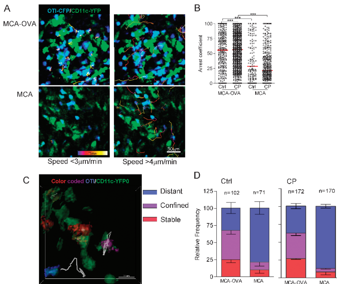
Figure 3. OTI T cells make Ag-dependent interactions with TuDCs. (A) Representative TPLSM images of OTI T cells (cyan) and YFP + stromal cells (green) within an MCA tumor and an MCA-OVA tumor, 4 days after OTI-CFP T cell adoptive transfer in a CP-treated CD11c-YFP-transgenic mouse. Track paths of OTI T cell moving at the indicated mean velocity are shown colored according to the time of imaging (color-coded time bar is shown). (B) Quantification of OTI T cell arrest coefficient (MCA Ctrl, n = 137 ; CP, n = 419 and MCA-OVA Ctrl, n = 271 ; CP, n = 920 ). Mann-Whitney statistical significances are indicated (upper right). (C) Volume rendering reconstruction image shows three representative OTI T cells colored according to the type of interaction performed with YFP + cells. OTI T cell track paths are represented in white. (D) Quantification of the relative frequency of the three types of OTI T cell/YFP + cell interactions. Bars represent mean \pm SD of the relative frequency of the three types of interactions in each movie (three to four different movies have been evaluated for each condition). Total numbers of OTI T cell characterized are indicated.
