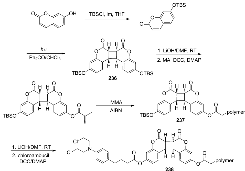
Scheme 108. Photorelease via [2 + 2]-Cycloreversion 417
