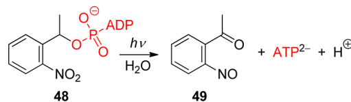
Scheme 31. Photochemistry of P 3 -1-(2-Nitrophenyl)ethyl Ester of Adenosine Triphosphate 156
