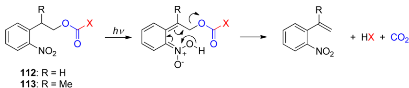
Scheme 43. Photolysis of 2-Nitro-2-Phenethyl Derivatives 226
