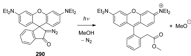
Scheme 134. Photochemistry of Caged Rhodamine (a Wolff Rearrangement) 517
