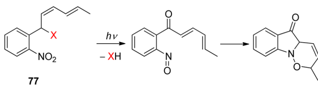
Scheme 37. Trapping of the Nitroso Byproduct in a Diels–Alder Cycloaddition 199
