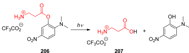
Scheme 87. Liberation of \beta -Alanine from the Aminonitrophenyl Chromophore 364
