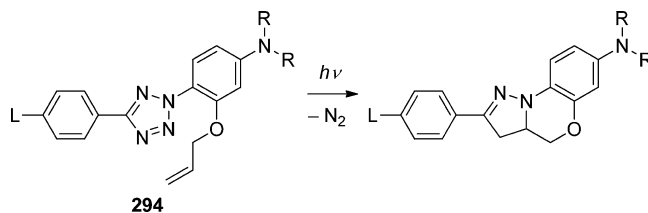
Scheme 137. Intramolecular Photoclick Reaction 526
