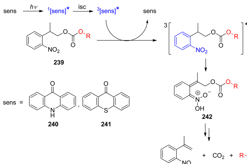
Scheme 111. Intramolecular Triplet Sensitization of the 2-(2-Nitrophenyl)propyl Chromophore
