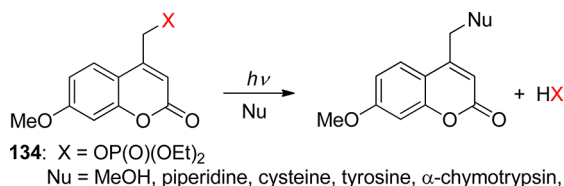
Scheme 49. Release of Phosphates from 7-Methoxycoumarin Derivatives 266
