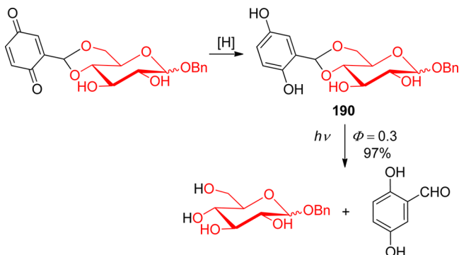
Scheme 80. Photolabile Protection of Glycols 339
