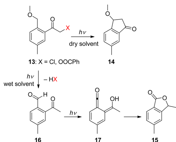
Scheme 10. Photochemistry of 2,5-Dimethylbenzoyl Oxiranes 71
