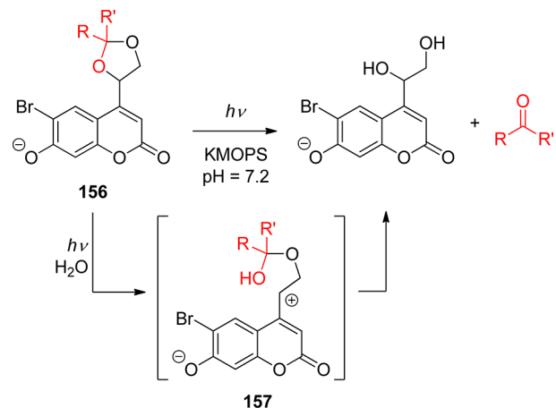
Scheme 59. Photorelease of Coumarin-Caged Carbonyl Compounds 287,291
