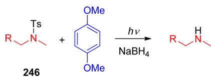
Scheme 114. Photosensitized Fragmentation of Tosylamides 422
