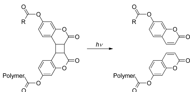
Scheme 108. Photorelease via [2 + 2]-Cycloreversion 417
