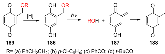
Scheme 79. Photolabile Benzylidene Protection of Carbohydrates 340
