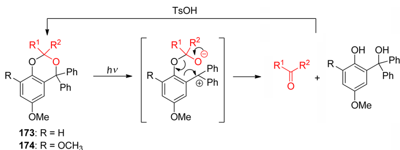
Scheme 69. Photolabile Acetals for the Protection of Ketones and Aldehydes 320
