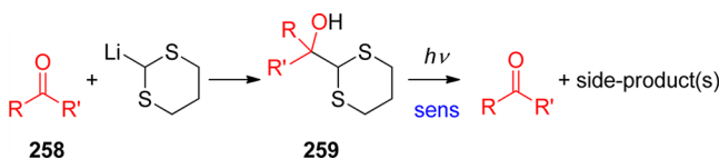
Scheme 123. Photochemistry of Dithiane Moiety 443
