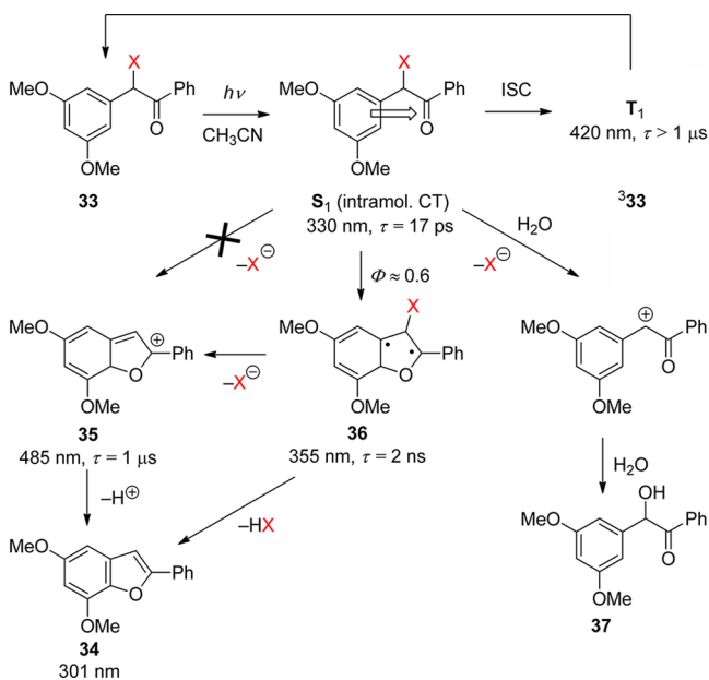
Scheme 24. Mechanism of the Photocyclization of 3',5'-Dimethoxybenzoic (DMB) Derivatives (X = OCOR, OPO(OEt) 2 , F) 122,123b
