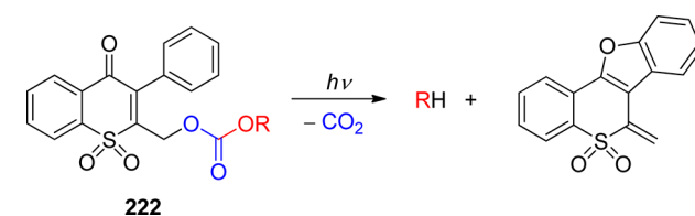
Scheme 98. Photochemistry of a Thiochromone S,S-Dioxide Derivative 403
