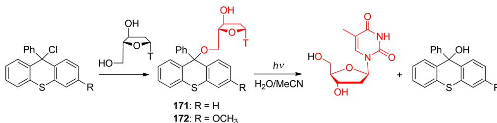
Scheme 69. Photolabile Acetals for the Protection of Ketones and Aldehydes 320
