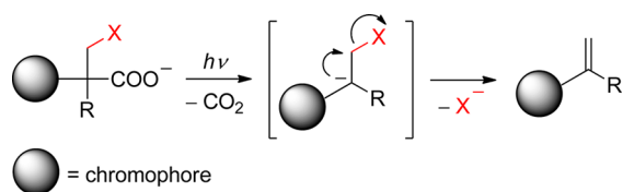
Scheme 91. Carbanion-Mediated Photocleavage
