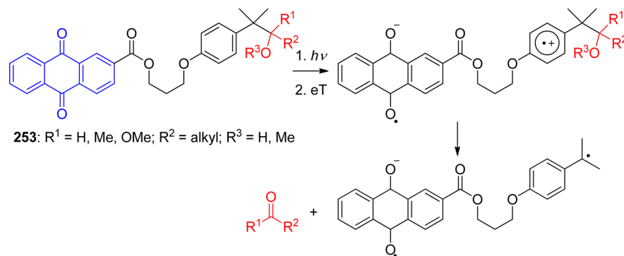
Scheme 121. Intramolecular Sensitization of the Phenethyl Alcohol/Ether Group 440
