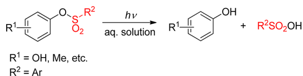
Scheme 88. Photochemistry of Arylsulfonyl Esters
