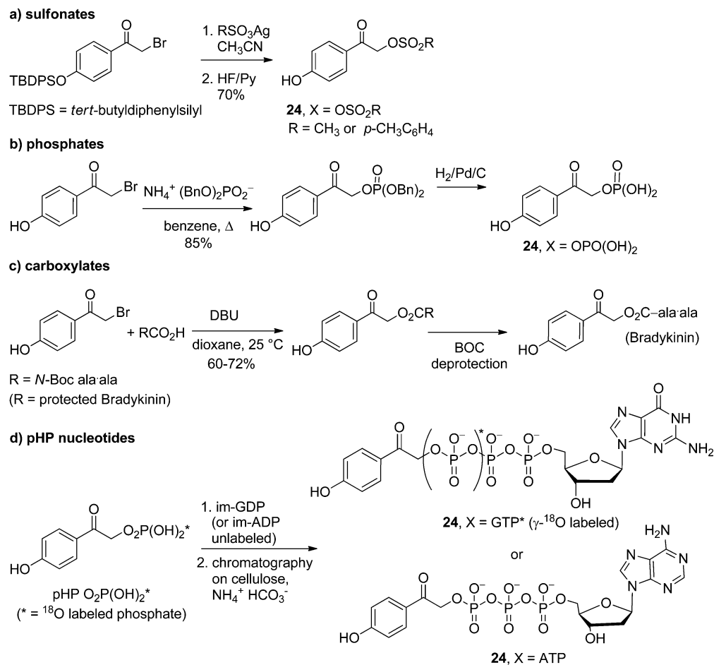
Scheme 17. Strategies for \alpha -Diazo- p -Hydroxyacetophenone Coupling to Protect Acidic Leaving Groups 93
