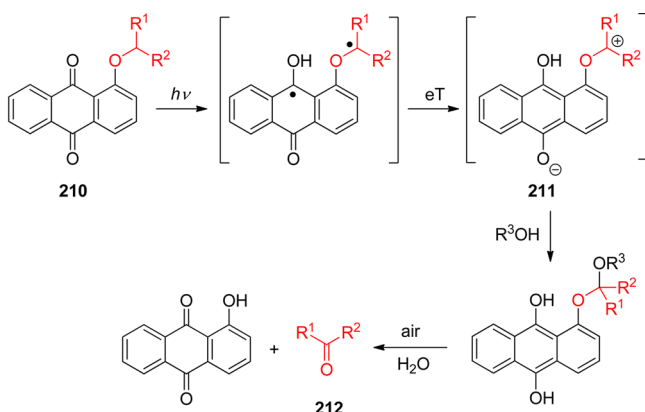
Scheme 91. Carbanion-Mediated Photocleavage
