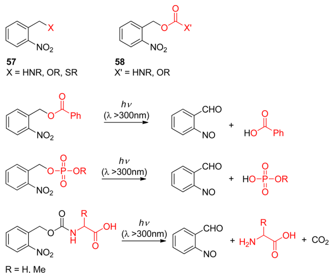
Scheme 34. Photolysis of Some o -Nitrobenzyl Derivatives
