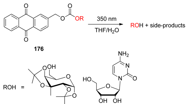
Scheme 71. Aqmoc Caging of Primary Alcohols 324,326d
