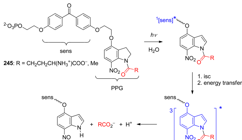
Scheme 112. Antenna-Sensitized 1-Acyl-7-nitroindoline System 247,248
