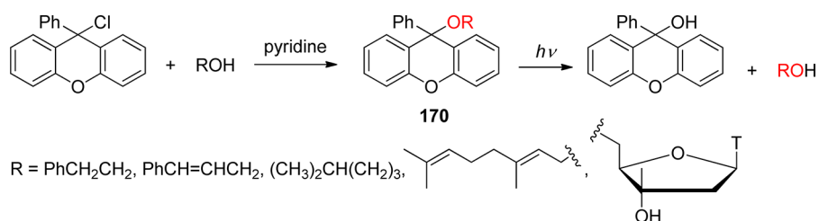
Scheme 68. Use of the S-Pixyl PPG for Caging and Release of Nucleosides 318
