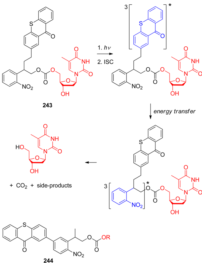
Scheme 111. Intramolecular Triplet Sensitization of the 2-(2-Nitrophenyl)propyl Chromophore
