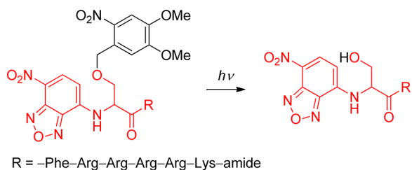
Scheme 132. Fluorescent Reporter of Protein Kinase Activity 515
