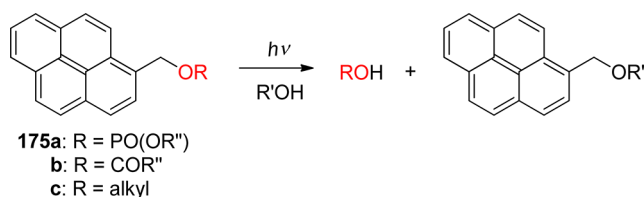
Scheme 70. Photocleavage of the Fluorescent (Pyren-1-yl)methyl Protecting Group 326
