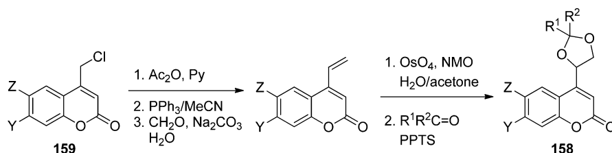
Scheme 61. Photoactivation of Coumaryl-Caged Progesterone 310
