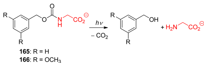
Scheme 63. Uncaging of Glycine 1,311
