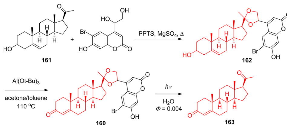
Scheme 61. Photoactivation of Coumaryl-Caged Progesterone 310
