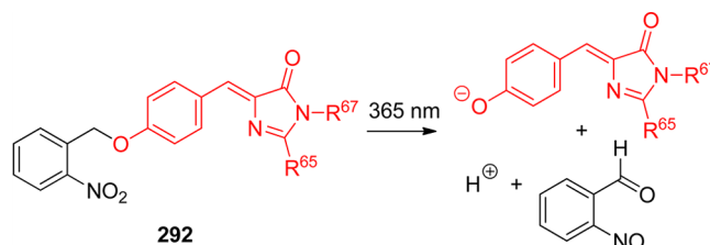
Scheme 136. o -Nitrobenzyl-Caged GFP 519
