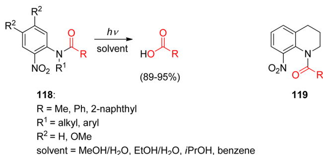
Scheme 44. Photoactive o -Nitroanilide Derivatives 241
