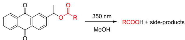
Scheme 72. Aqe Cage for Carboxylic Acids 328
