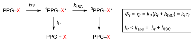
Scheme 1. Simple Case Where the Release Rate Constant of the Free Substrate (Leaving Group) X, k_r , Is Smaller than Its Appearance Rate Constant, k_{\text{app}}
