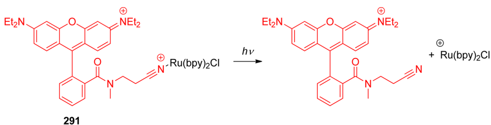
Scheme 135. Photochemistry of Caged Rhodamine 356
