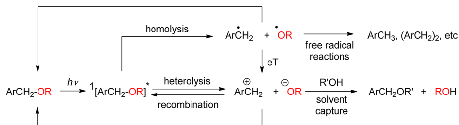
Scheme 64. Photochemistry of Arylmethyl Ethers
