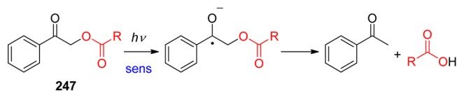
Scheme 115. Photosensitized Release of Carboxylic Acids from Phenacyl Esters 430
