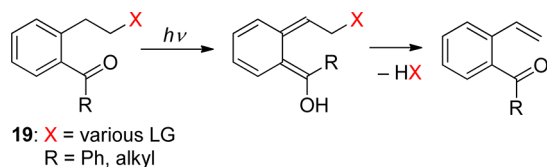
Scheme 11. Photochemistry of 1-[2-(2-Hydroxyalkyl)phenyl]ethanones 74
