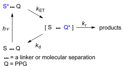
Scheme 109. Photoinduced Energy Transfer (Blue Color Depicts an Electronic Excitation)
