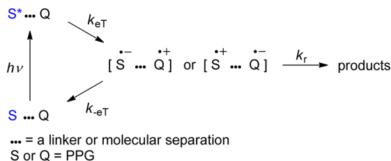
Scheme 113. Photoinduced Electron Transfer (Blue Color Depicts a Sensitizer)
