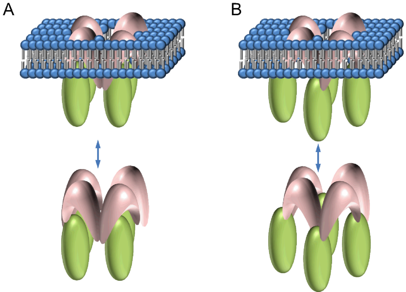
FIGURE 9. Two versions of the hetero-octameric model proposed for the quaternary structure of the Wzm-Wzt ABC transporter. A. Four units of Wzm interacting with four units of Wzt face-to-face. B. Four units of Wzm are interlaced with four units of Wzt.
