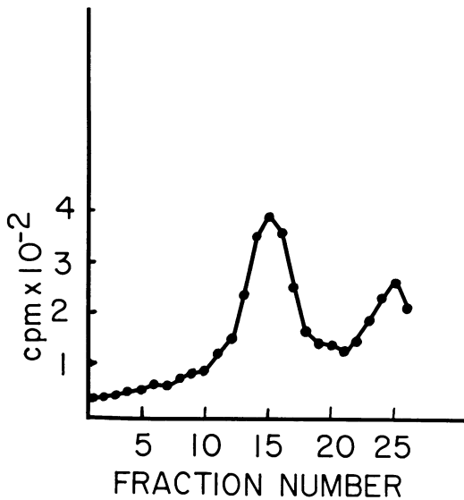
FIG. 4. Sucrose gradient centrifugation of ^3\text{H} -labeled visna virus RNA under low ionic strength. The RNA was extracted from purified visna virus labeled with ^3\text{H} -uridine and centrifuged through a sucrose gradient containing 0.001\text{ M NaCl} and 0.001\text{ M EDTA} as detailed in Materials and Methods and in Fig. 2.
