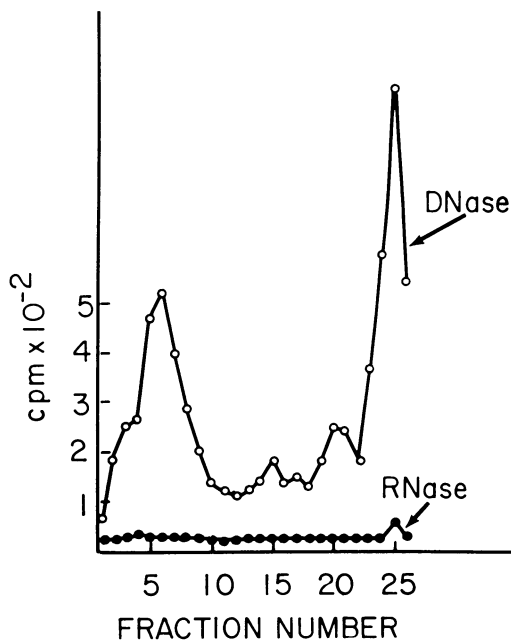
FIG. 3. Sucrose gradient centrifugation of ^{32}\text{P} -labeled extract after treatment with ribonuclease and deoxyribonuclease. The ^{32}\text{P} -labeled extract from purified visna virus was dissolved in TM buffer. Two 0.2-ml samples of the solution were each incubated with ribonuclease (50 \mu\text{g}/\text{ml} ) and deoxyribonuclease (50 \mu\text{g}/\text{ml} ) at room temperature for 30 min and then centrifuged through sucrose gradients as detailed in Materials and Methods and in Fig. 2.
