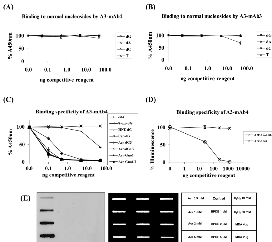
Figure 3. Specificity of mAbs by competitive ELISA and Slot-Blotting
