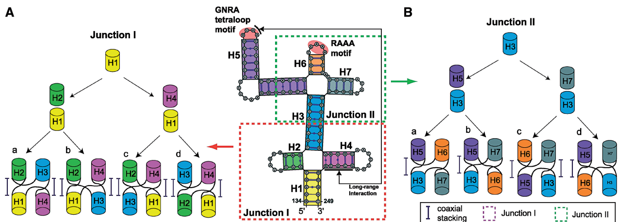
Figure 3. Piecing the possible helical arrangements for the two four-way junctions in domain 3 of IRES. (A) Possible junction topologies of junction I with two coaxial stacking following the 5'- to 3'-direction: (a) H_1H_4 and H_2H_3 without crossing in the single-stranded region, (b) H_1H_4 and H_2H_3 with crossing, (c) H_1H_2 and H_3H_4 with crossing and (d) H_1H_2 and H_3H_4 without crossing. (B) Predicted junction topologies of junction II with one or two coaxial stacking following the 5'- to 3'-direction: (a) H_3H_5 and H_6H_7 without crossing, (b) H_3H_5 and H_7H_6 with crossing, (c) H_5H_6 and H_7H_3 without crossing and (d) H_6H_5 and H_7H_3 with crossing.
