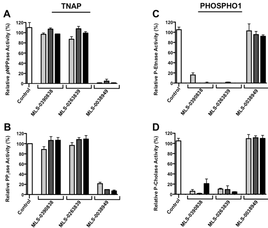
Fig. 3. Selectivity of PHOSPHO1 and TNAP inhibitors
