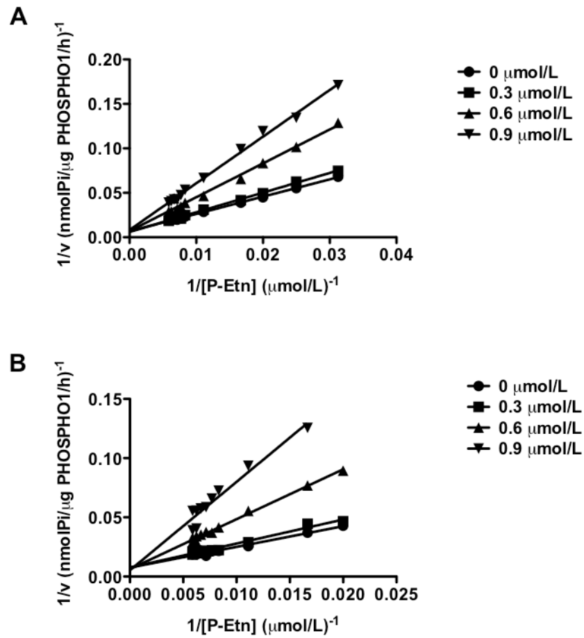
Fig. 2. Mode of action of PHOSPHO1 inhibition by lansoprazole and MLS-0263839 Double reciprocal plots of PHOSPHO1 activity versus the concentration of the PHOSPHO1 substrate P-Etn (32 – 170 μmol/L), in the presence of increasing concentrations of lansoprazole (A) and MLS-0263839 (B). Results are presented as mean ± S.E.M.
