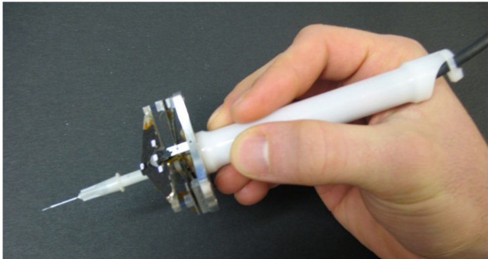
Fig. 1. Micron, a handheld micromanipulator.
