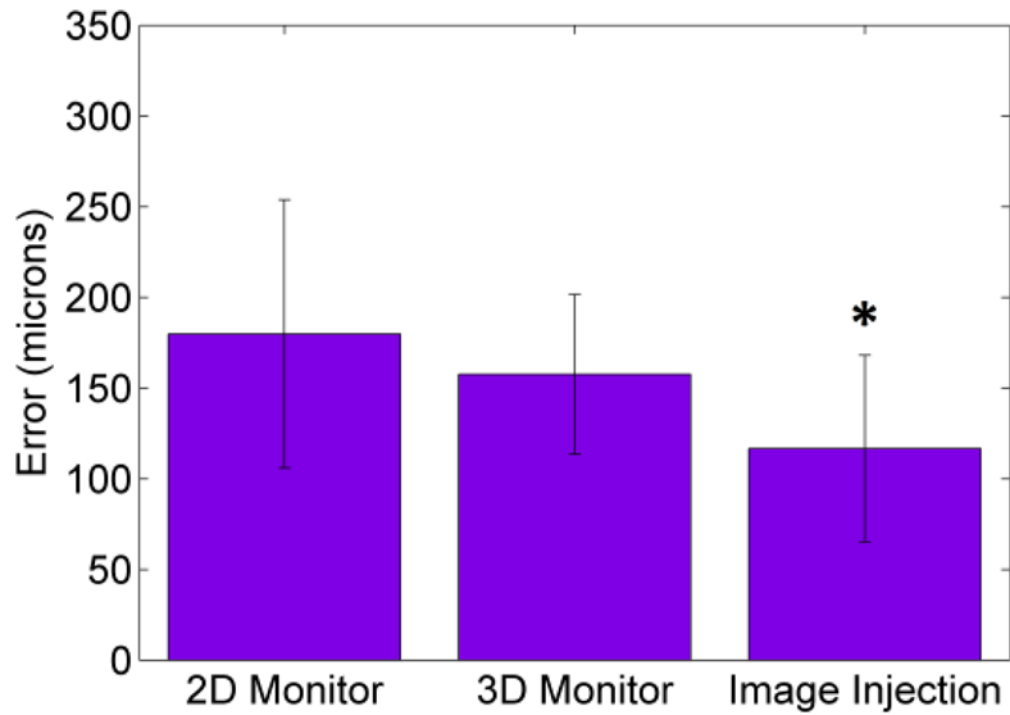
Fig. 8. Novices' maximum 3D error with error bars for standard deviation, across 24 trials with each display. Image injection significantly reduces error compared to 2D and 3D monitor ( p < 0.05 ).
