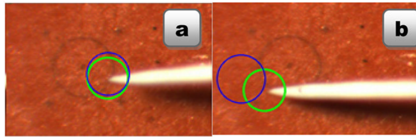
Fig. 6. Circle-tracing task with visual cues: green represents the goal, blue the null position of the manipulator. (a) Coincidence of the circles is the desired condition, indicating Micron is near the center of its range of motion. (b) The position and size of the blue circle indicate the planar and depth error, respectively.
