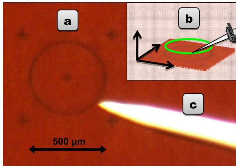
Fig. 5. (a) Circular target, 500 \mu\text{m} in diameter, on a rubber surface. (b) Generating a 3D circle virtual fixture from the tracked target. (c) White-painted, tapered tip of Micron.
