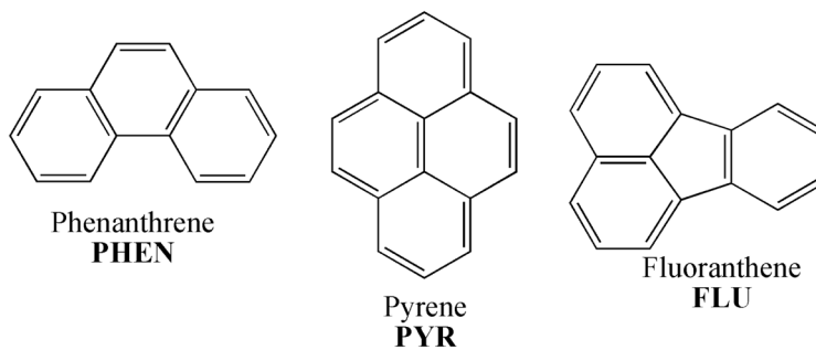
Fig. 1. Chemical structures and abbreviations for the quinones and polycyclic aromatic hydrocarbons tested for DTT activity.
