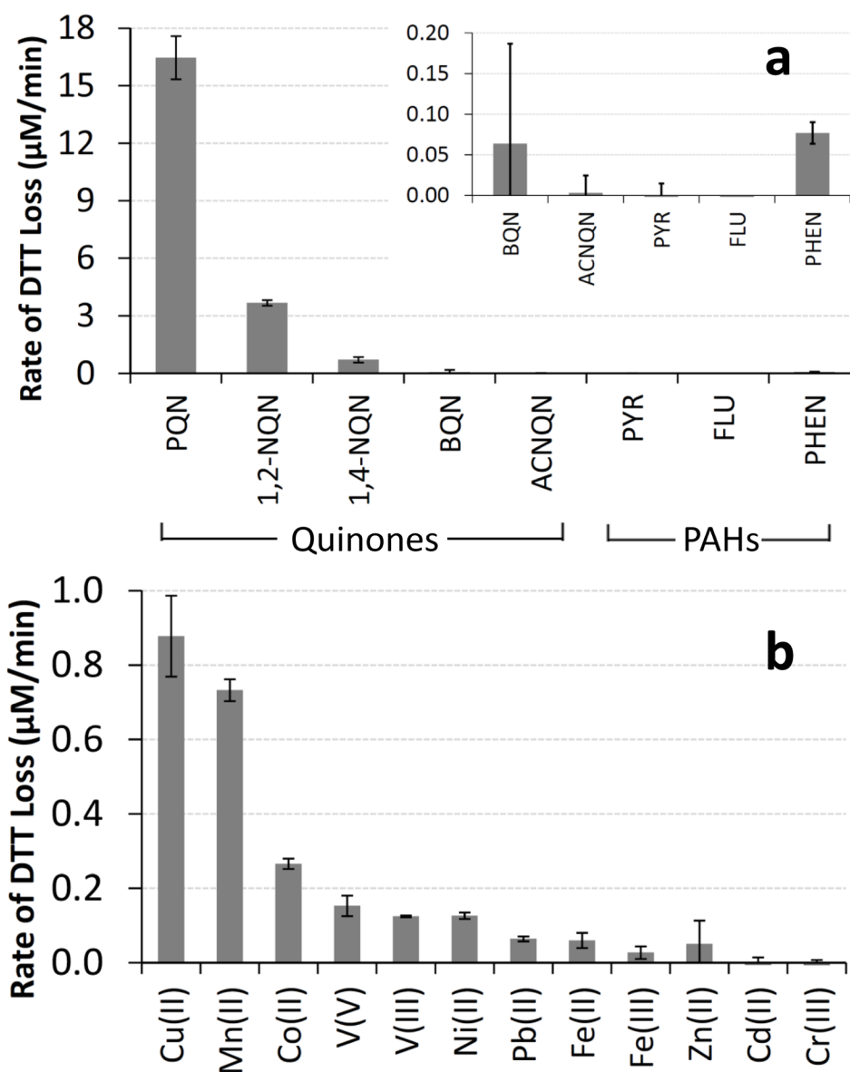
Fig. 3. Blank-corrected rates of DTT loss from five quinones and three PAHs ( a ) and from 12 transition metals ( b ). The concentration of each species was 1 \mu\text{M} , except for BQN which was 0.93 \mu\text{M} , 1,4-NQN which was 1.21 \mu\text{M} and Cd(II), which was 5 \mu\text{M} .
