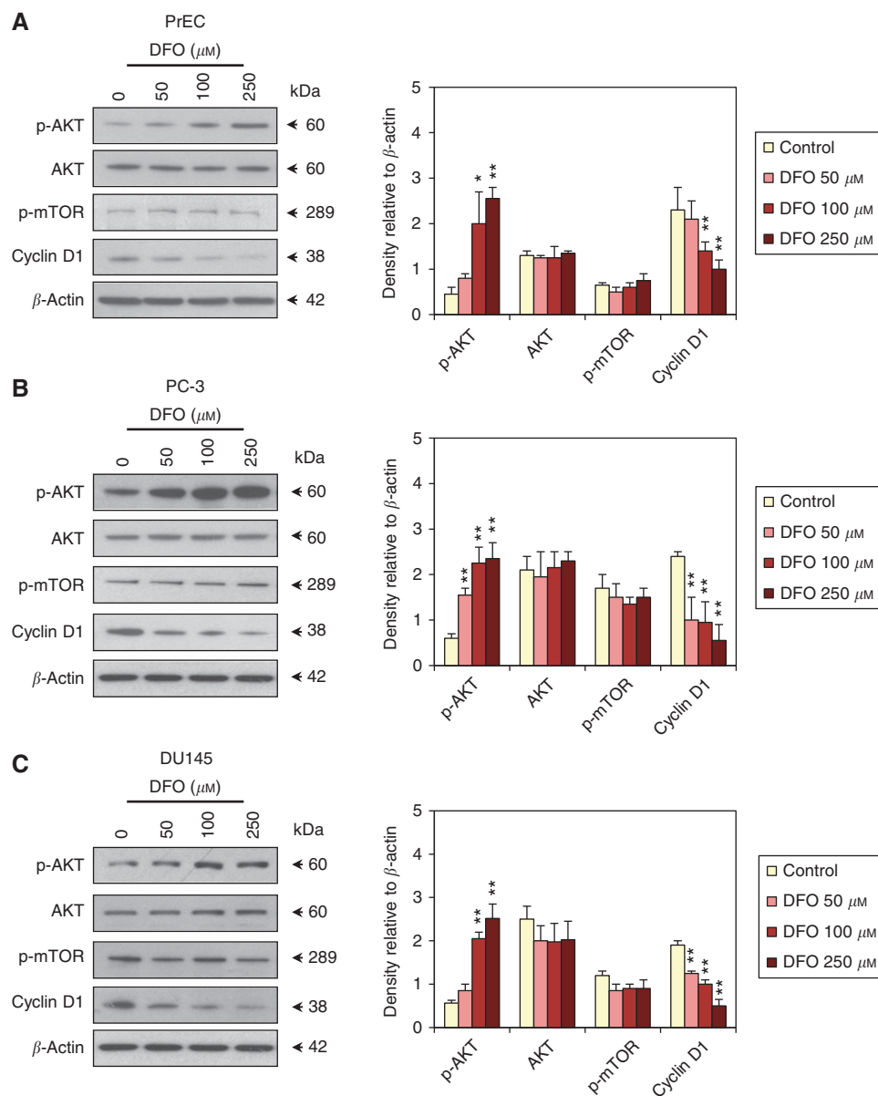
Figure 3. Incubation of cells with DFO (50, 100 and 250 \mu\text{M} ) increases p-AKT (Ser 473 ) levels, but in terms of its effect on downstream effectors, has no effect on p-mTOR (Ser 2448 ), while decreasing cyclin D1 expression in (A) PrEC, (B) PC-3 and (C) DU145 cells after 24 h at 37 °C. Western blots are typical of three independent experiments, with densitometric analysis representing mean \pm s.d. Relative to control: * P < 0.05 , ** P < 0.01 .
