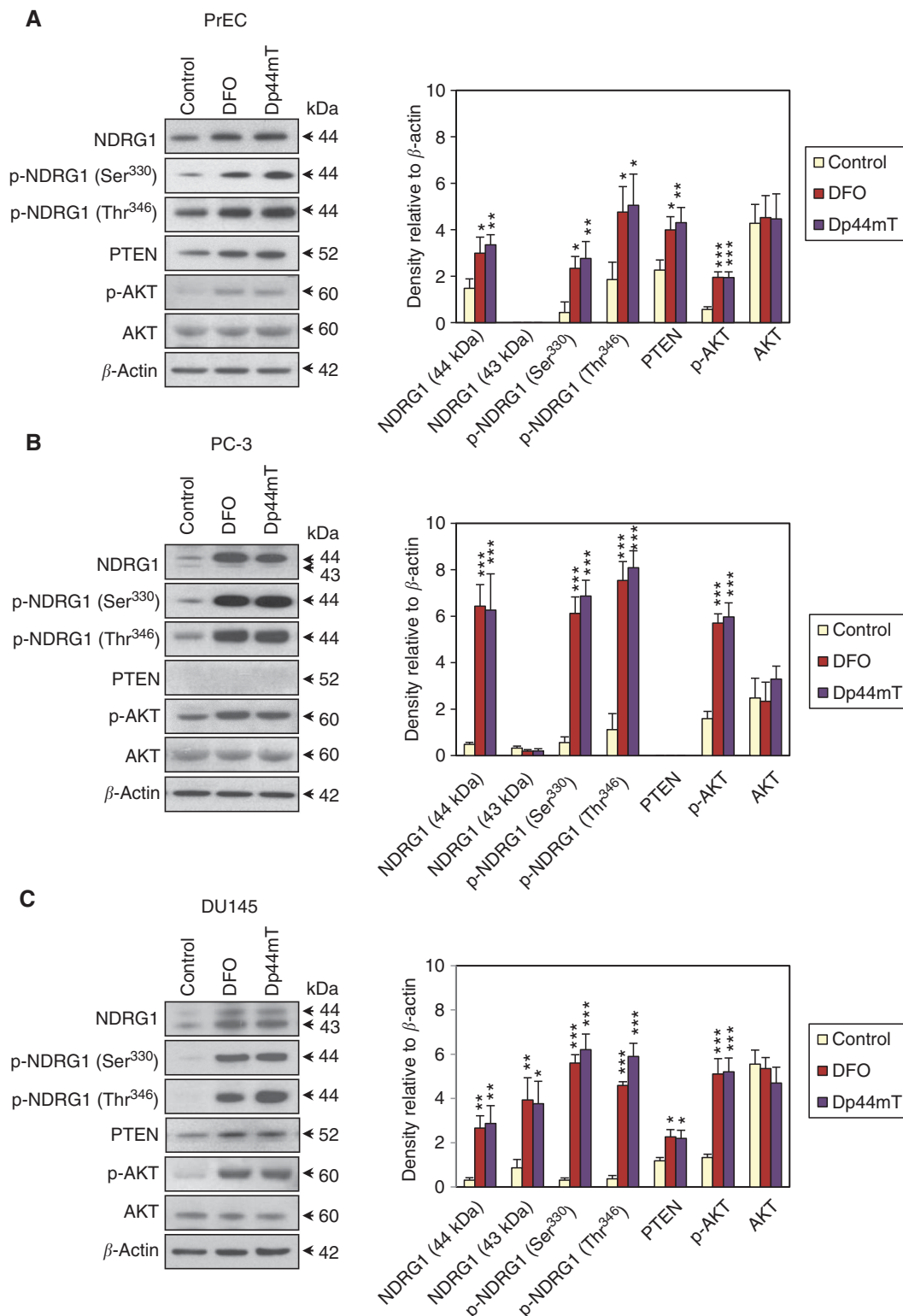
Figure 1. Increase of NDRG1, p-NDRG1 (Ser 330 ), p-NDRG1 (Thr 346 ), PTEN, p-AKT (Ser 473 ) and AKT protein levels in (A) PrEC, (B) PC-3 and (C) DU145 cells after a 24 h incubation at 37 °C with control medium, DFO (250 μM) or Dp44mT (2.5 μM). Western blots are typical of three independent experiments, with densitometric analysis representing mean ± s.d. Relative to control: *P<0.05, **P<0.01, ***P<0.001.
