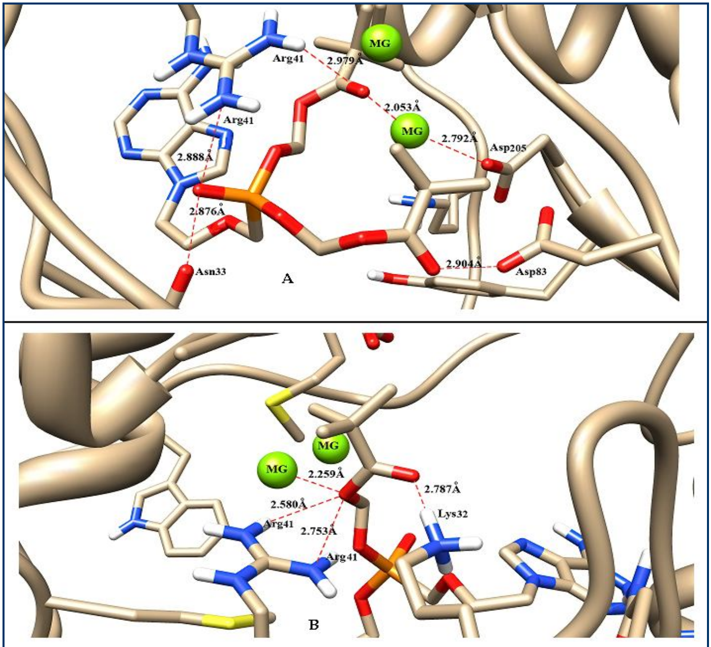
Figure 1: Impact of HBV rtI233V mutation and adefovir binding. Binding conformation of A ) wild type (rtI233) and B ) mutant (rtI233V) protein-ligand complex derived from Autodock. The ligand (adefovir) and interacting residues are shown in stick format and red dotted lines represent H-bond. The image was prepared using Chimera 1.6.2 software.
