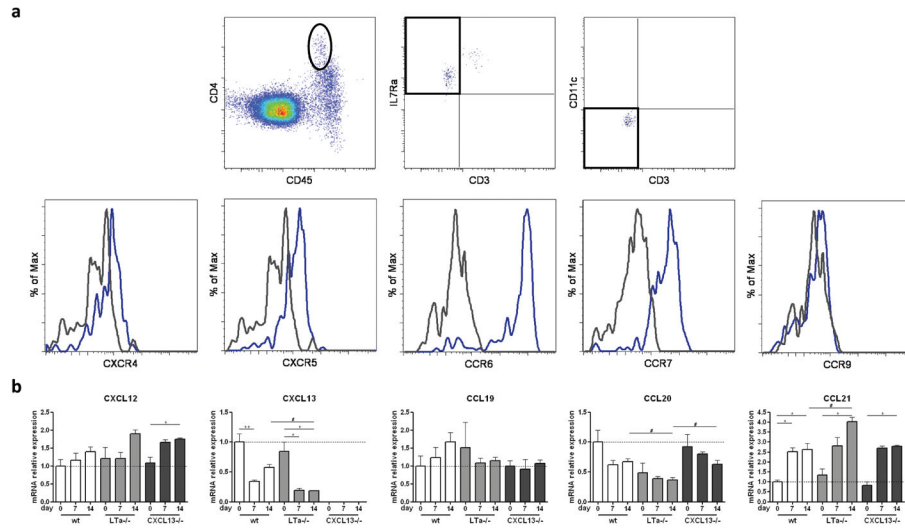
Figure 4. Chemokine receptor expression on colonic LTi cells and colonic chemokine expression a Chemokine receptor expression on CD45 int CD4 + IL7R \alpha + CD3 - CD11c - cells LTi cells was assessed by flow cytometry. Grey histograms represent FMO controls in which the primary antibody was omitted, while blue histograms represent the actual staining. At least 8 colons were used per analysis and a representative FACS experiment is shown. The experiment was performed 3 times. b Chemokine mRNA expression in whole colons of wild-type, LTA -/- and CXCL13 -/- mice of different ages was assessed by real-time PCR. 4–7 colons were analyzed per group. The expression of each transcript in each sample was normalized to the expression of the transcripts for the housekeeping genes Cyclophilin and Ubiquitin. The mean expression levels of each transcript for sample wild-type day 0 were arbitrarily set at 1. Data were compared with one way non-parametric ANOVA and Dunn’s multiple comparison tests. Mean \pm SEM is shown. * p<0.05, ** p<0.01 between different age groups within the same mouse genotype; # p<0.05 between different mouse genotypes within the same age group.
