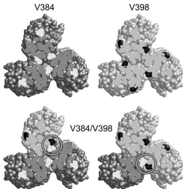
Fig. 2. Proximity reporters for the trimer of dimers. Cross sections (viewed from the tip) show the four possible trimer combinations of dark-gray dimers with V384C (white) and light-gray dimers with V398C (black) (Tsr residue numbering). In the crystal structure, the shortest distance between \alpha -carbons at the 384 positions is 11.4 Å; the shortest distance between \alpha -carbons at the 398 positions is 13.8 Å. In mixed trimers that contain both V384C and V398C dimers, a reporter pair (circled) should form at the trimer interface. The distance between their \alpha -carbons is 6.2 Å.
