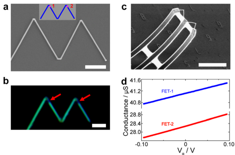
Figure 4. Parallel nanoFET KNWs
