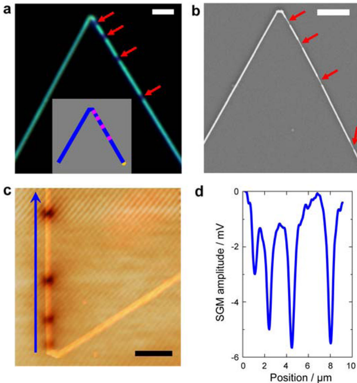
Figure 3. Series nanoFET in V-shaped KNWs
