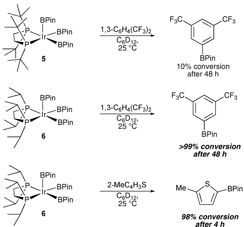
Scheme 3. Relative reactivities of 5 and 6 with 1,3-bis(trifluoromethyl)- benzene and 6 with 2-methylthiophene at 25^\circ\text{C} .
