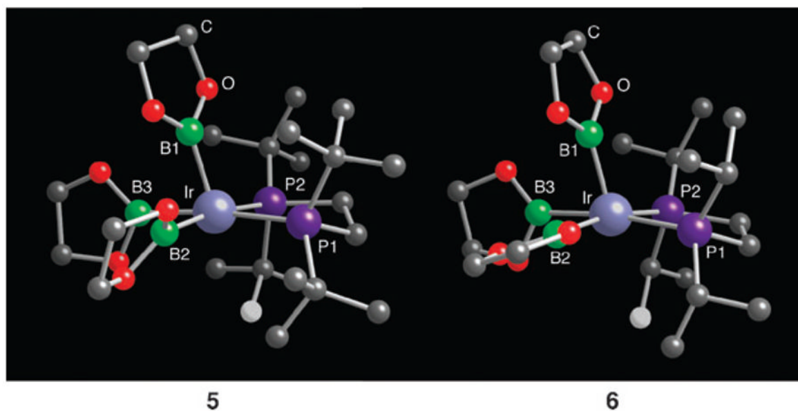
Fig. 1. X-Ray structures of compounds 5 and 6 with BPin methyl groups omitted. The white carbons are those with the closest Ir contacts ( \text{Ir}\cdots\text{C} = 3.169 \text{ \AA} in 5 and 3.419 \text{ \AA} in 6 ). In both cases, the Ir-C distances are significantly longer than those in compounds with Ir C-H agostic interactions.
