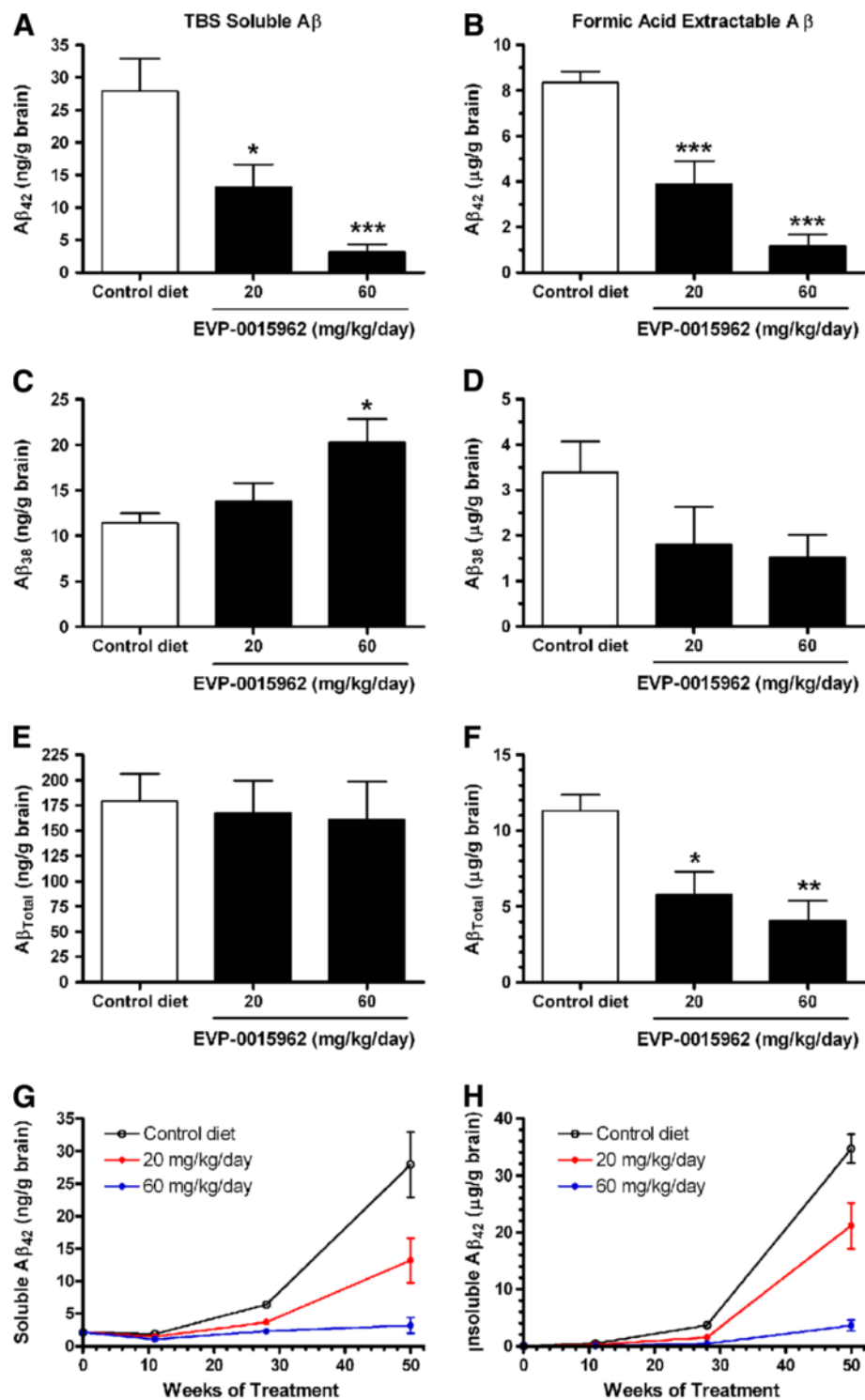
Figure 7 Chronic daily exposure to EVP-0015962 in Tg2576 mice reduces A \beta peptide levels. A-F . TBS soluble ( A, C, E ) and formic acid extractable ( B, D, F ) A \beta peptide levels determined by ELISA from the brains of Tg2576 mice after 50 weeks of treatment with EVP-0015962 for A \beta_{42} ( A-B ), A \beta_{38} ( C-D ), and A \beta_{Total} ( E-F ). N = 5 mice per group. Differences from the control diet group: * p < 0.05 , ** p < 0.01 , *** p < 0.001 (1-way ANOVA, post-hoc Newman-Keuls test). G-H . A \beta_{42} peptide levels measured at the beginning of treatment and after 11, 28, and 50 weeks of treatment with EVP-0015962, showing the time course of accumulation of A \beta_{42} . G . TBS soluble A \beta_{42} . H . Insoluble A \beta_{42} . At 11 and 28 weeks, insoluble A \beta_{42} was extracted with only formic acid. At 0 and 50 weeks, the 4-step procedure was used, and the insoluble fraction is the sum of the A \beta_{42} extracted with Triton ® -X, SDS, and formic acid. N = 4–6 mice per group and time point. Graphs illustrate mean \pm SEM.
