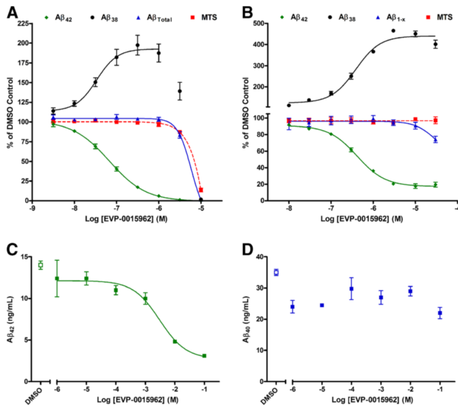
Figure 2 EVP-0015962 is a potent \gamma -secretase modulator. A. Concentration response curves for A \beta 42 , A \beta 38 , and A \beta Total determined by enzyme-linked immunosorbent assay (ELISA), and for cell viability in the H4-APP 751 cell assay. IC 50 = 67 nM for A \beta 42 and EC 50 = 33 nM for A \beta 38 . For cell viability determined using the MTS assay, IC 50 = 5.56 \mu M. IC 50 > 3 \mu M for A \beta Total . For A \beta 38 , the EC 50 value is determined for the concentration range of 3 nM to 1 \mu M of EVP-0015962, to avoid the portion of the curve where toxicity is observed. N = 6 independent experiments. B. Concentration response curves for A \beta 42 , A \beta 38 , and A \beta 1-x determined by ELISA in media and for MTS from rat primary neocortical cultures. IC 50 = 427 nM for A \beta 42 and EC 50 = 384 nM for A \beta 38 . IC 50 > 30 \mu M for A \beta 1-x and the MTS assay. N = 4 independent experiments for A \beta 42 , A \beta 1-x , and MTS and 2 for A \beta 38 . C. Concentration response curve for A \beta 42 in the cell-free assay. IC 50 = 3.9 \mu M. D. Concentration response curve for A \beta 40 in the cell-free assay. In the cell-free assays, A \beta was determined by AlphaLISA in triplicate. All data are expressed as mean \pm standard error of the mean (SEM). For some data points, error bars are smaller than the sizes of the data points.
