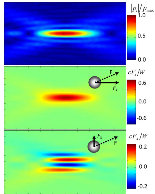
FIG. 2. (Color online) Spatial distributions in the xz plane of the amplitude of the incident pressure wave (top), the radiation force axial component F_z (middle), and the lateral component F_x (bottom) when the sphere is positioned on the x axis for the source shown in Fig. 1. The image box size is 20 \times 10 mm. Note the sphere is included for scale and is not in fact fixed in only the shown position.
