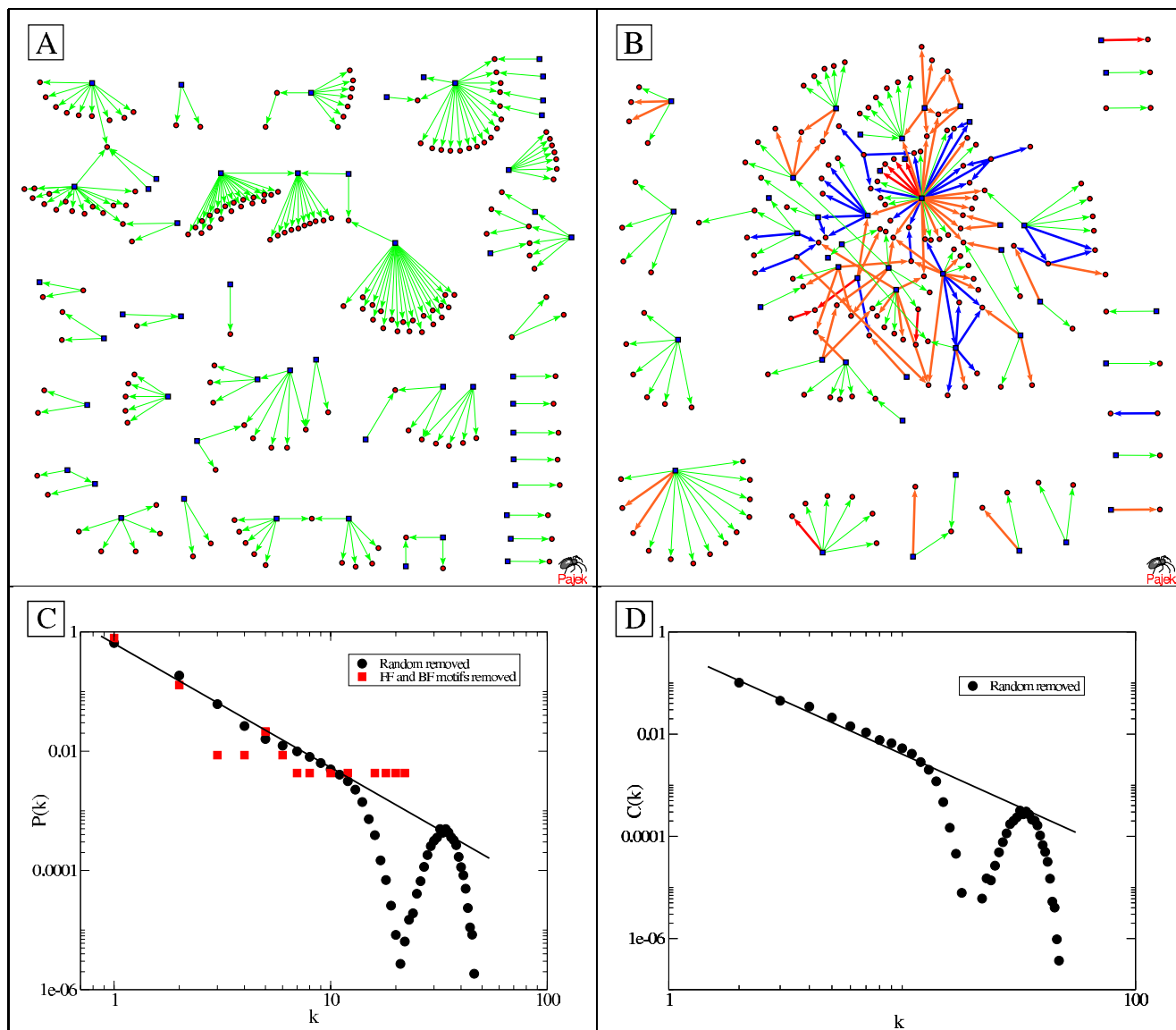
Figure 3 Network fragmentation under random- or targeted link removal. a. We have removed the links among nodes of the FF and BF motif clusters from the original network. b. The same number of links as in (a) are removed randomly. In order to determine qualitatively the difference between removing the links of FF and BF motif cluster and randomly removing the same number of links, we have determined (c) the connectivity distribution, P(k) , and (d) the clustering distribution, C(k) of the remaining networks. The distributions for random removal of links have been averaged over 5000 different samples. The solid line in panel c has slope \gamma = -2 , and is the best fit for the random link removal. The solid line in panel d has slope \tau = -2 . We do not show C(k) for the network in panel a, since the clustering coefficients for all nodes by definition are zero. The deviation from the solid line in panels c,d, are caused by the TF, crp , which represent the most connected node of the network.
