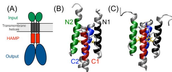
Figure 1. Position and structures of a canonical HAMP domain in the signaling complex. (A) Schematics of canonical HAMP connected to input and output domain; (B) Side view of the structure of wild-type Af1503-HAMP, (C) Side view of the A291F variant. The color code indicates the helix: black - N1, N-terminal helix of Monomer 1; red - C1, C-terminal helix of Monomer 1; green - N2, N-terminal helix of Monomer 2; blue - C2, C-terminal helix of Monomer 2; orange - residues with mutation; Colored helical residues are used in the calculation of the helical RMSD and helical properties.
