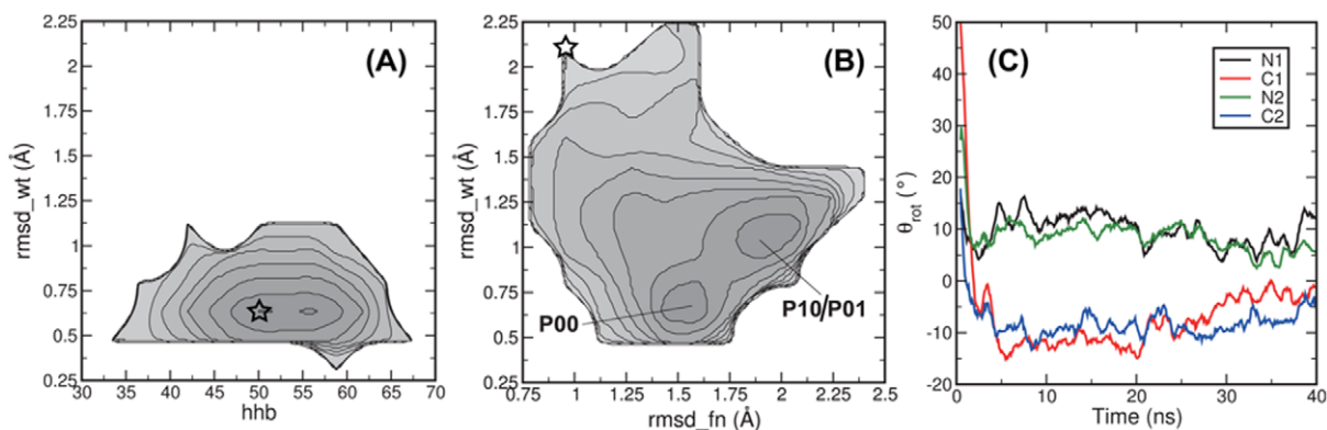
Figure 2. RMSD from experimental structures and helical rotation. The negative log of the probability distributions are shown for (A) the WT system as a function of the number of helical hydrogen bonds hhb and the RMSD with respect to the NMR structure of WT, rmsd_{wt} and (B) the WT* system as a function of the RMSD with respect to the NMR structure of the A291F mutant, rmsd_{fn} and rmsd_{wt} . Labels indicate stable states. Contour lines are rendered every 1k_B T . The stars indicate the starting point of the simulations. (C) Time evolution of helical rotation in the WT* system. The helical rotation for each helix is plotted as a function of simulation time, as a running average of 10 ps for a typical WT* simulation. The helical rotation is calculated as the angle between a reference point on the helix, the center of mass of the helix and the reference point on an aligned reference structure, see Methods for details. The MD simulations show that HAMP can visit additional conformational states.
