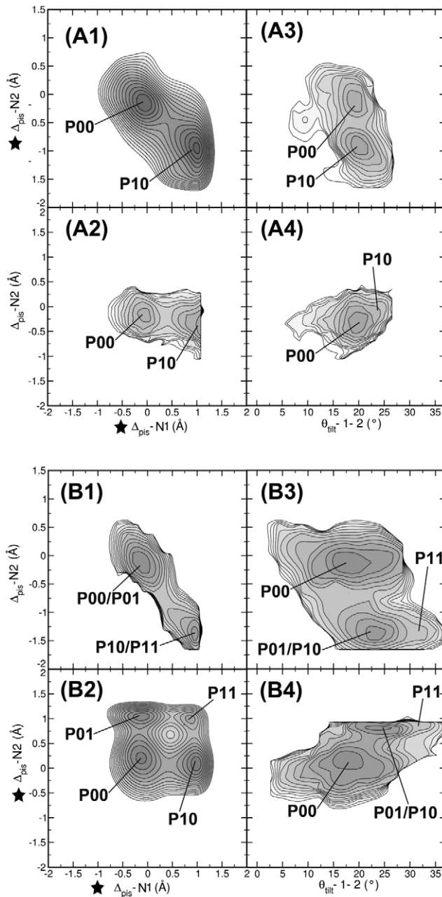
Figure 6. Two dimensional bias on piston motions. In the metadynamics simulations the biasing potential was applied to (A) \Delta_{pis}-N1 and \Delta_{pis}-C2 ; (B) \Delta_{pis}-N1 and \Delta_{pis}-N2 . The results are shown as free energy profiles in the following projections: (A1,B1) \Delta_{pis}-C2 versus \Delta_{pis}-N1 ; (A2,B2) \Delta_{pis}-N2 versus \Delta_{pis}-N1 ; (A3,B3) \Delta_{pis}-C2 versus \theta_{tilt}-1-2 ; (A4,B4) \Delta_{pis}-N2 versus \theta_{tilt}-1-2 . (A1) and (B2) show the free energy landscapes of biased CVs, the other subplots are corresponding reweighted free energy surfaces. Stars indicate the CV on which the bias was applied. Labels indicate stable states. Contour lines are rendered every 1k_B T . The two-dimensional metadynamics simulations show that the piston motions of helices N1 and C2 are oppositely correlated, and that this correlation also exists for the C1,N2 pair. doi:10.1371/journal.pcbi.1002913.g006
