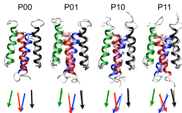
Figure 4. The four states of HAMP: P00, P10, P01, P11. Ribbon representations and schematic representations of the four states, with black N1; red C1; green N2; blue C2. Conformation P00 is rendered transparent in the depictions of states P01 , P10 and P11 to illustrate the differences.
