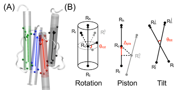
Figure 8. Definition of helical motions. (A) Positions of four consecutive C_\alpha atoms, indicated by colored spheres (black N1; red C1; green N2; blue C2) are used to define the head and tail groups. The green points at the head. (B) Three collective variables (CVs) describing helical motions: rotation \theta_{rot} , piston shift \Delta_{pis} and tilt \theta_{ilt} . Reference vectors are indicated in gray. The CV definitions are indicated in red. See main text for an explanation of the definitions. doi:10.1371/journal.pcbi.1002913.g008
