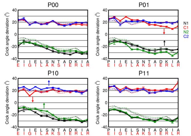
Figure 7. Deviation of the ideal Crick angles for the four piston states. The Crick angle deviation is plotted as a function of residue in the N and C-helices for the P00, P10, P01 and P11 states. The error bars indicate the variation over 40 snapshots. The dashed lines represent the Crick angle deviations as measured for the NMR structure of wild-type Afl503-HAMP (PDB-code 2L7I). There are little differences between the states. doi:10.1371/journal.pcbi.1002913.g007
