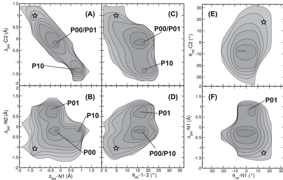
Figure 3. Piston shift, tilting and rotation of helices in WT* trajectories. The negative log of the probability distributions are plotted for (A) \Delta_{pis} - C2 versus \Delta_{pis} - N1 ; (B) \Delta_{pis} - N2 versus \Delta_{pis} - N1 ; (C) \Delta_{pis} - C2 versus \theta_{tilt} - 1 - 2 ; (D) \Delta_{pis} - N2 versus \theta_{tilt} - 1 - 2 ; (E) \theta_{rot} - C2 versus \theta_{rot} - N1 ; (F) \Delta_{pis} - N1 versus \theta_{rot} - N1 . The labels indicate stable states. Contour lines are rendered every 1k_B T . The stars indicate the starting point of the simulations. The WT* simulations reveal that the different conformational states of HAMP can be distinguished by differences in piston shift and tilt angle.
