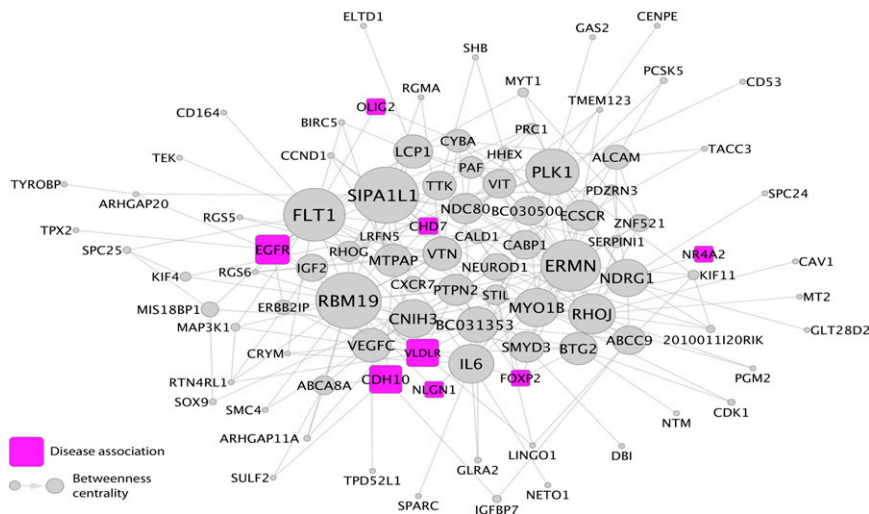
Fig. 4. Gene coexpression network. Coexpression network of genes differentially expressed in SP, with annotation for disease-implicated genes (FDR <5%).
