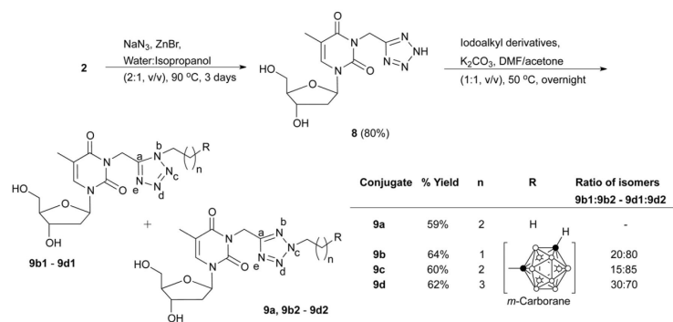
Scheme 3. Synthesis of N3-tetrazolylmethyl-type dThd derivatives ( 9a , 9b1/2-9d1/2 ).
