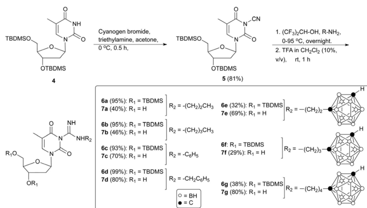
Scheme 2. Synthesis of N3-guanidine-type dThd derivatives ( 7a-7g ).
