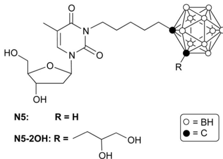
Figure 1. Structures of N5 and N5-2OH.
