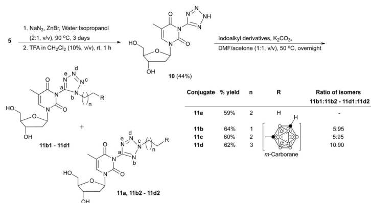
Scheme 4. Synthesis of N3-tetrazolyl-type dThd derivatives ( 11a , 11b1/2-11d1/2 ).
