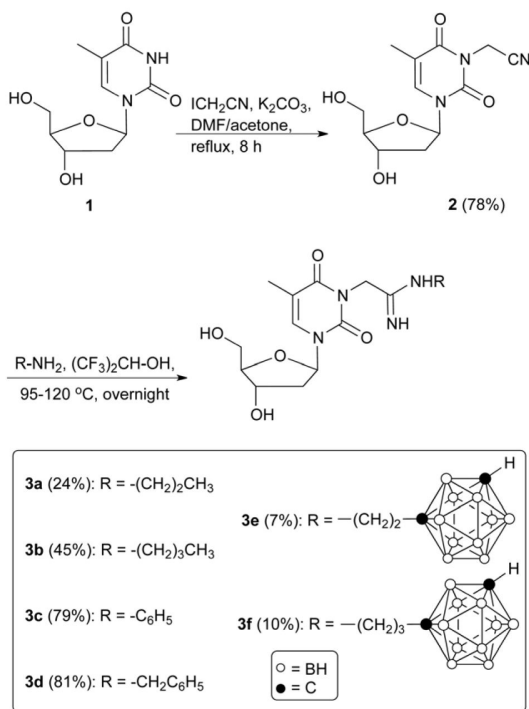
Scheme 1. Synthesis of N3-amidine-type dThd derivatives ( 3a-3f ).
