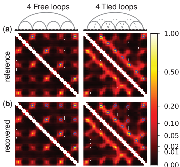
Figure 4. Heat maps representing (a) reference and (b) recovered CPs for a chain of 45 beads with (left) four free loops or (right) four tied loops. Free loops result from connecting loop end-beads with harmonic restraints (gray arcs in top-left schematic), while tied loops result from connecting middle beads across free loops (dotted arcs in top-right schematic). Blue circles on the maps identify pairs of beads that were restrained (a) when generating reference CPs and (b) when performing the ensemble recovery procedure. Test systems with two and three loops (Table 2) yielded a similarly good visual match between reference and recovered CP maps (data not shown).
