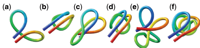
Figure 3. Energy-minimized conformations of the test systems used to generate reference CPs for validating the proposed computational method. The systems are labeled as in Table 2. Images were generated using UCSF Chimera (48).
