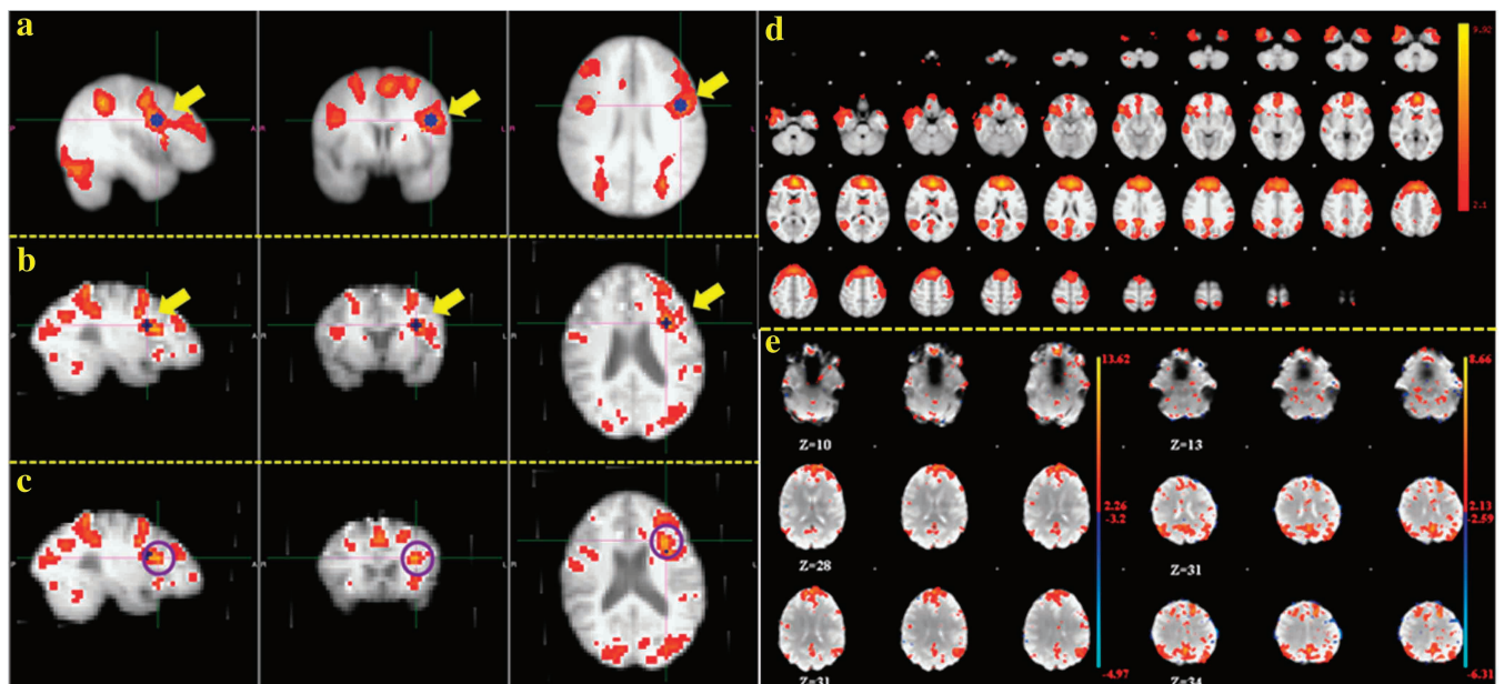
Figure 3. (a–c) Illustration of manual selection of working memory ROIs for an individual with the guidance of group activation map. (a) Group-wise activation map. The ROI considered is shown in blue and highlighted by yellow arrow. (b) Individual activation map. The registered ROI peak from group activation map is shown in blue and highlighted by yellow arrow. (c) The manually chosen ROI peak for this individual. The ROI peak is the cross of 2 axes and the center of the highlighted purple circle. (d and e) Identification of DMN using ICA. (d) group-ICA result of DMN; (e): 2 individual samples of ICA maps for DMN.
