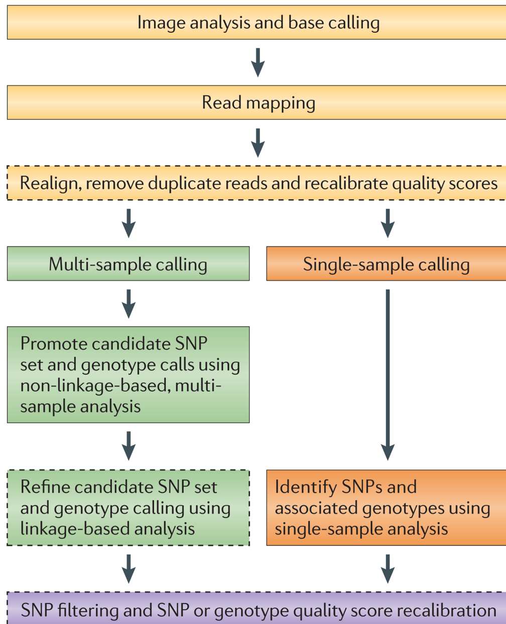
Figure 1. Steps for converting raw next-generation sequencing data into a final set of SNP or genotype calls
