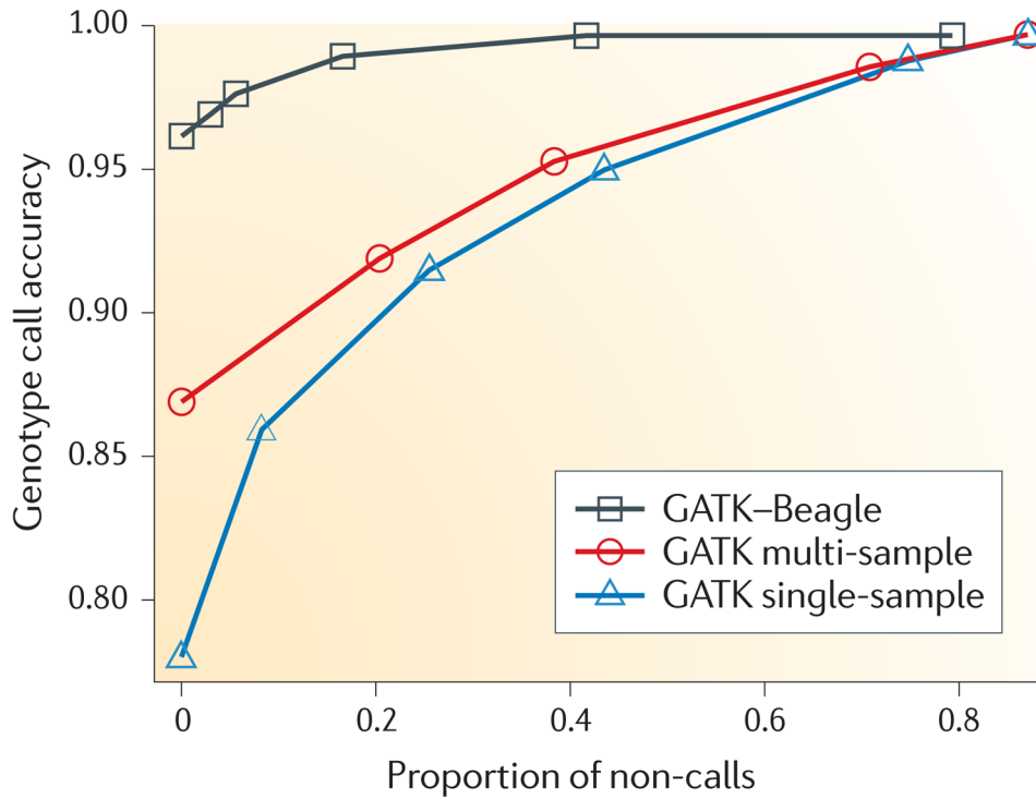
Figure 2. A comparison of three genotype callers
