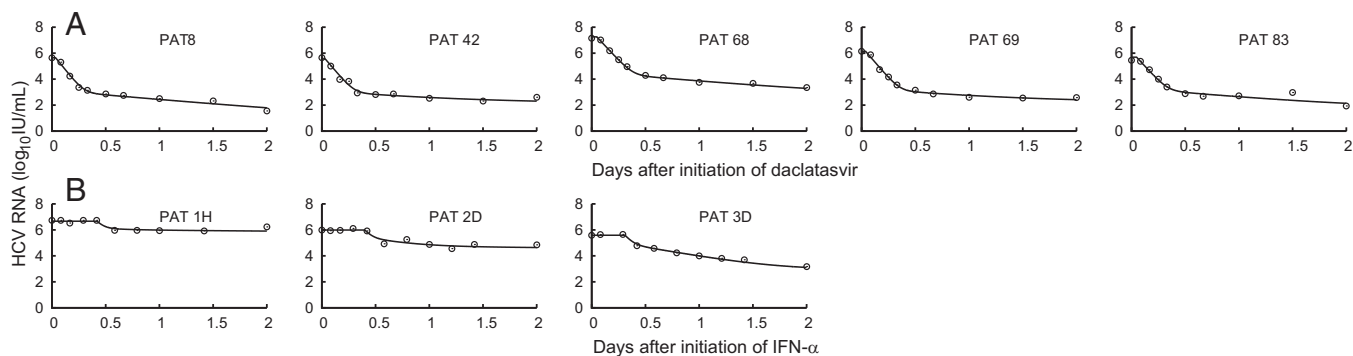
Fig. 1. Viral kinetics and model predictions. Viral load data ( \circ ) and standard and multiscale models' predictions (solid line) for (A) five patients receiving one dose (four received 100 mg and one, Pt42, received 10 mg) of daclatasvir (BMS-790052) and (B) three representative patients receiving daily IFN- \alpha of 5 MIU (Left), 10 MIU (Center), and 15 MIU (Right). Although interpretations are different, the model curves of the standard model (Eq. 1) and of the multiscale model (Eq. 3) overlap and cannot be distinguished.
