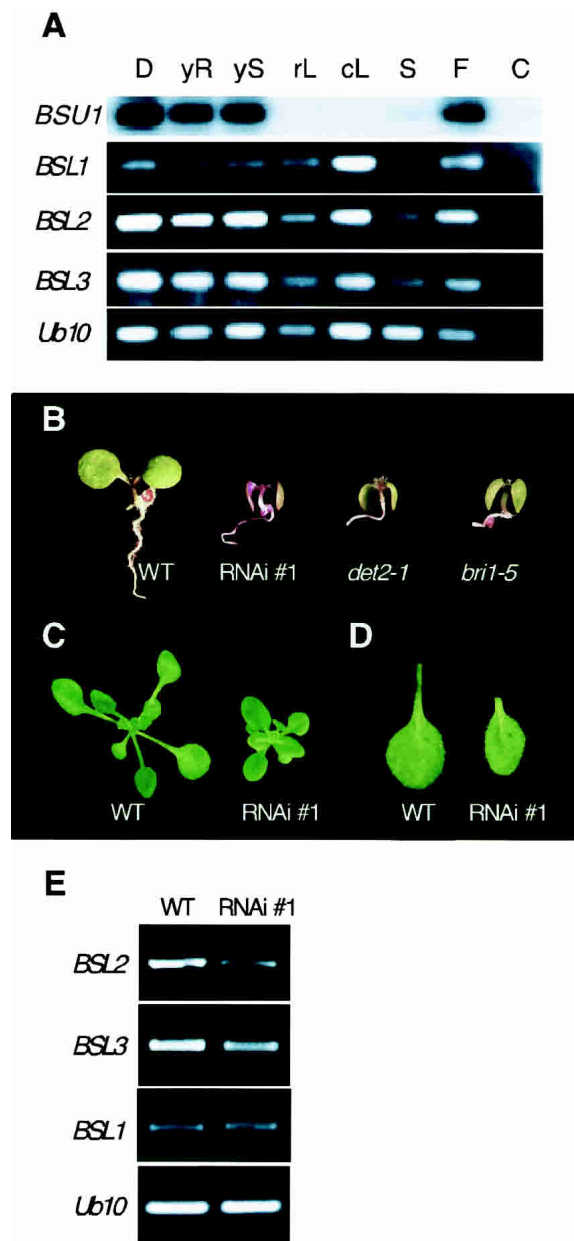
Figure 7. Functional redundancy in the BSU family. (A) Expression pattern of BSU1 and its homologs evaluated by RT-PCR in Ws-2 . (D) Five-day-old seedlings grown in the dark; (yR) roots of 12-day-old seedlings grown in the light on vertical plates; (yS) shoots of 12-day-old seedlings grown in the light on vertical plates; (rL) mature rosette leaves; (cL) mature cauline leaves; (S) mature stem; (F) the tip of the inflorescence, including flowers at different developmental stages; (C) negative control with no template added. (B) Phenotype of 10-day-old seedling of Ws-2 (WT), RNAi knockdown T2 plants for BSL2 and BSL3 , det2-1 and bri1-5 , grown under long-day conditions. (C) Rosette phenotype of 20-day-old WT and RNAi plants. (D) Comparison of the first true leaves in WT and RNAi plants. (E) Expression analysis by RT-PCR of BSL1 , BSL2 , and BSL3 in both WT and RNAi plants. Ubq10 serves as a control.
