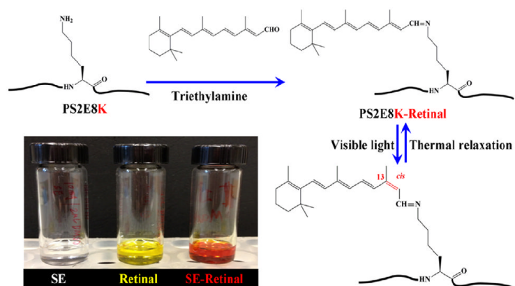
Figure 2. Schematic for retinal modification of the lysine residues in the silk-elastin copolymer PS2E8K. Insert: Chemical reactions for PS2E8K before and after retinal modification (Left: PS2E8K in DMSO solution; Middle: retinal molecules in DMSO solution; Right: retinal-modified PS2E8K in DMSO solution).
