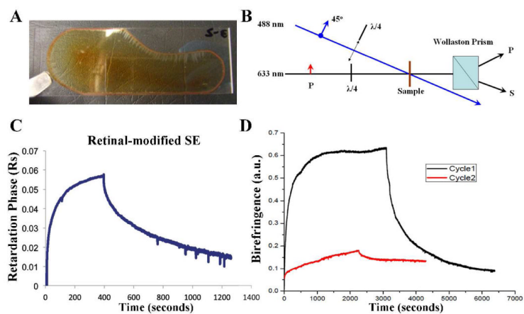
Figure 6. Optical polarization of retinal-modified polymer films. A. Retinal-modified PS2E8K film dried onto a glass slide. B. Birefringence measurement setup. The birefringence written using a 488-nm argon ion laser beam polarized at 45°
