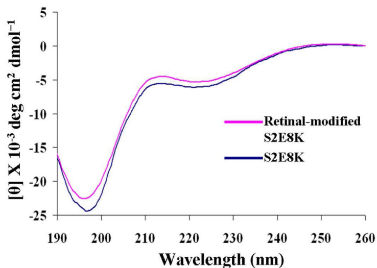
Figure 5. Far-UV CD spectra of unmodified and retinal-modified silk-elastin copolymer PS2E8K. All spectra were recorded at room temperature (25°C) using a 0.5 mm path-length quartz cell with protein concentrations of 0.5 mg/ml.
