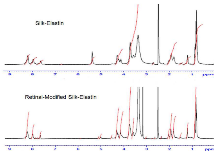
Figure 3. 1 H-NMR analysis of silk-elastin-like polymers before (upper panel) and after (lower panel) retinal modification.
