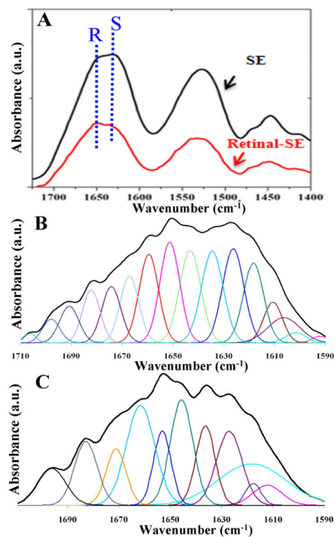
Figure 4. Structure characterization of unmodified and retinal-modified silk-elastin polymer PS2E8K by FTIR. A. FTIR spectra. R represents random coil, S for beta-sheet structure. B & C. Selected FTIR absorbance spectra of unmodified (B) and retinal-modified (C) silk-elastin copolymer in the amide I' regions after Fourier self-deconvolution. The heavy line represents the deduced absorbance band. The light lines represent the contributions to the amide I' band.
