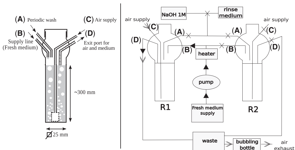
FIG. 1. —Left: Diagram of a single reactor during the culture stage. The reactor has been assembled by glass blowing, and incorporates a square cross-section glass tube in the bottom portion, and a screwed plastic cap on top. The entry and exit tubes are welded to the top of the reactor and comprise an air supply connected to a tube that is terminated by a porous glass plug at the bottom of the reactor (generating bubbles that give both aeration and mixing via air lift) (C), a fresh supply of medium (B), a wash fluid entry point (A), a fluid exit, and a biphasic mixture of air and liquid (D). Right: Schematics of the tubing connections during the culture phase in the reactor R1. R1 and R2 are the two reactors of the setup; each is temperature regulated; filtered air (rate adjusted by a flow meter/needle valve) is injected through port (C) of reactor R1. It passes through a porous glass plug and generates bubbles serving for both culture aeration and mixing via air lift within the reactor. The bottle containing the fresh medium is connected to a peristaltic pump; a constant flow of medium arrives at port (B) of reactor R1. A heating resistance heats the medium before entry (B), to prevent backward contamination of the supply of medium; the reactor wash solution (connected to port (A) and not used at this stage of operation of R1) comprises NaOH 1 M and rinse medium (the same solution as the supply of medium to the reactor); a waste bottle is connected to port (D) of reactor R1. It receives a biphasic mixture of air and medium exiting from the reactor by a common path and traps the liquid; the air exiting from the waste bottle is bubbled through bleach in a bubbling bottle, so as to avoid laboratory air contamination. The full arrows indicate the circulation of liquids, and the open arrows indicate the circulation of air. Crosses indicate the pinched-closed sections of tubes. Every week, the content of the operating reactor is transferred to the already cleaned tandem reactor. During the transfer phase (e.g., from R1 to R2), port (D) of R1 is closed and ports (A), (B), and (C) are open; ports (B) and (C) of R2 are closed and ports (A) and (D) are open. Air and medium containing bacteria come from R1 to R2 through port (A). When the transfer is stopped, R2 enters the culture phase, and R1 is rinsed and washed and ready for the next transfer.
