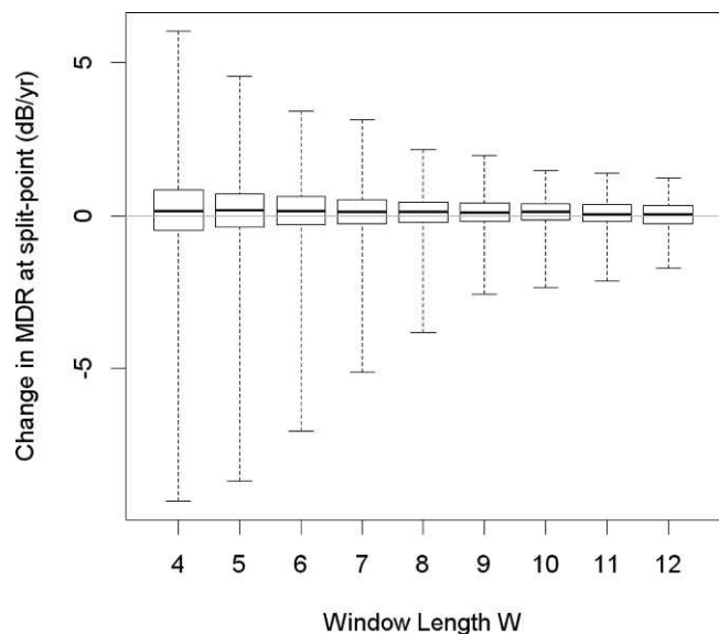
FIGURE 1. Box-and-whisker plots of the change in MDR occurring at the split-point, for different lengths of shortened window W . For each box, the central horizontal line represents the median value, the box covers the interquartile range, and the whiskers extend to the maximum and minimum values. The gray horizontal line indicates zero difference in MDR.
