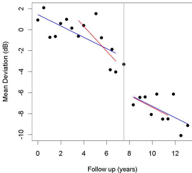
FIGURE 2. The series of VF test results for a sample participant in the Delayed Treatment Cohort. The vertical gray line represents the first visit at which the subject was receiving treatment. The blue lines show the rate of change of mean deviation from linear regression over the entire sequences, before the split-point and commencing at least 9 months after the split-point. The red lines show the equivalent rates of change derived using the shortened sequences, that is the last seven fields before the split-point and the first seven fields at least 9 months after the split-point. Before the split-point, the red line is steeper than the blue line, showing that use of the shortened sequence makes trend analysis more sensitive to the rapid rate of change that occurred over this period. A change in rate is apparent at treatment onset using the shortened sequence, but not using the entire sequence. Note that when the split-point was caused by the subject reaching an endpoint, all confirmation fields were included in the Before W sequence.
