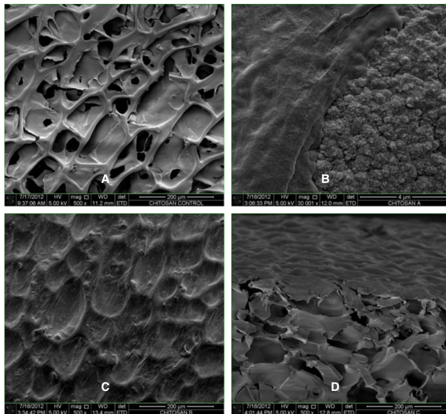
Figure 4 SEM micrograph of a 3-D culture of HDF into chitosan on day 14. Chitosan scaffold without cells. Scale bar 200 µm (A). Fibroblast proliferation into the chitosan. Scale bar 4 µm (B). Fibroblasts covering the pores. Scale bar 200 µm (C). Cross section. Scale bar 200 µm (D).
