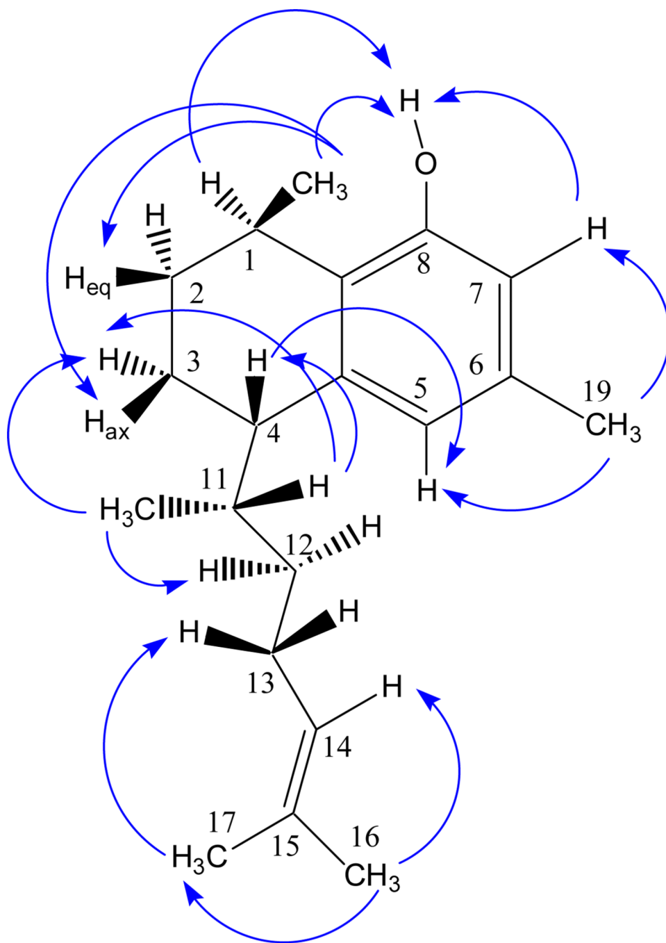
Figure 3. Observed NOE correlations for 1 .
