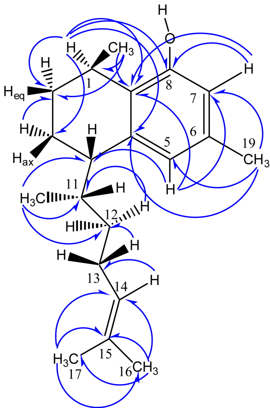
Figure 1. HMBC correlations found for 1 .
