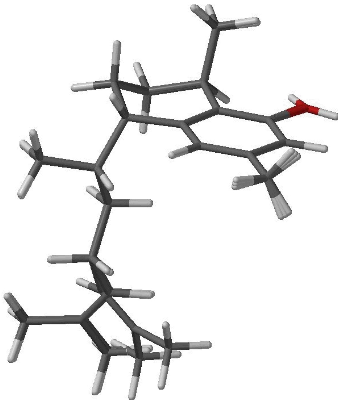
Figure 5. Superposition of the three low energy conformers of 1 , calculated by DFT//B3LYP/DGDZVP, accounting for 68.6% of the conformational distribution according to Table 2.
